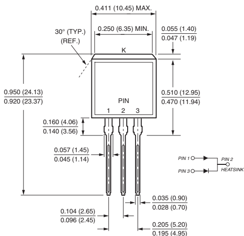
TO-262AA
