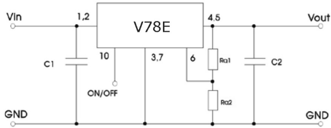
Application Circuit
