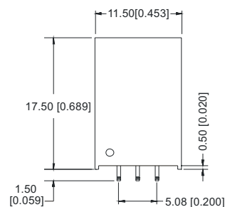
V78XX-1000R
