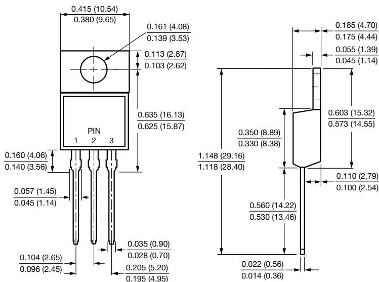
TO-220AB
