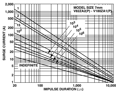
Figure 17 - V82ZA2(P) - V180ZA1(P)
