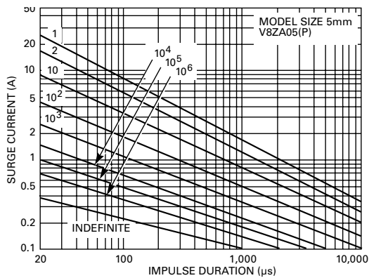
Figure 13 - V8ZA05P - V12ZA05P
