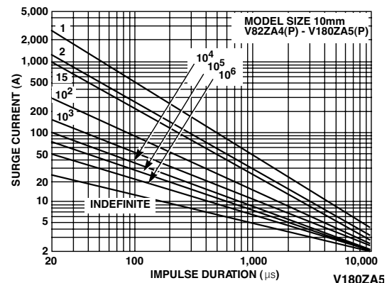
Figure 20 - V82ZA4(P) - V180ZA5(P)
