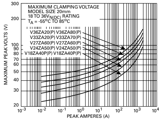
Figure 11 - V18ZA20(P) - V36ZA80(P)
