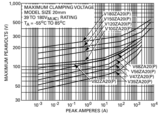
Figure 12 - V39ZA20(P) - V180ZA20(P)
