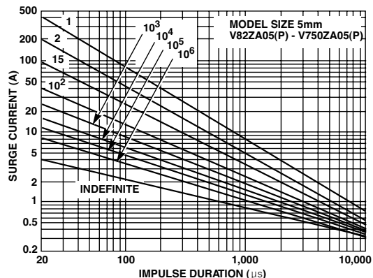
Figure 15 - V82ZA05(P) - V750ZA05(P)
