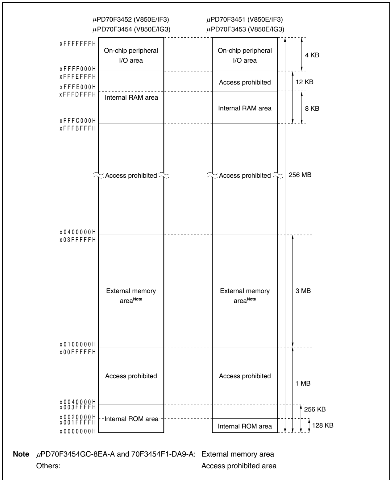
Figure 3-4. Memory Map
