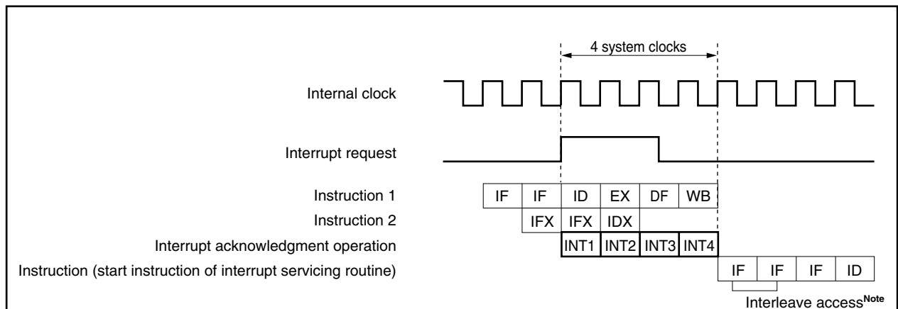
Figure 20-14. Pipeline Operation at Interrupt Request Acknowledgment (Outline)
