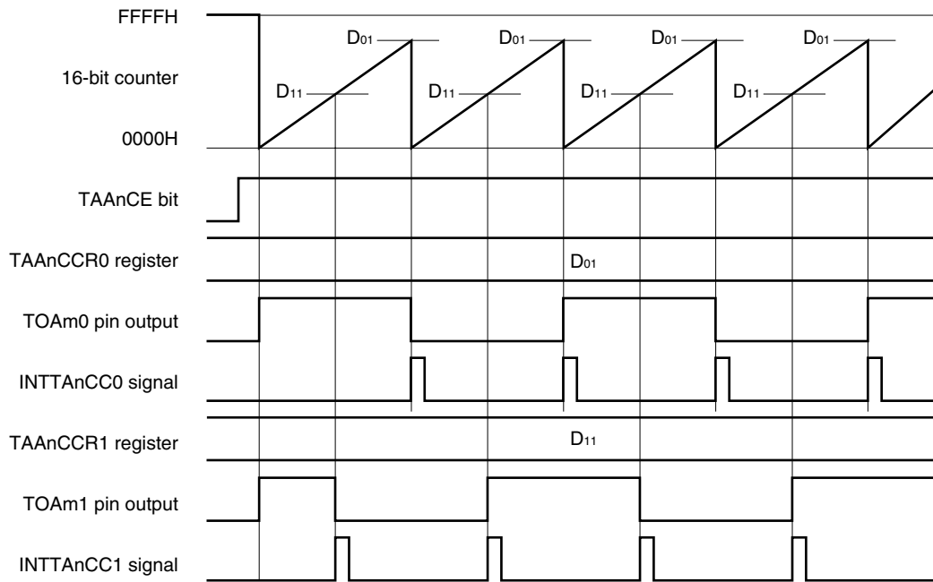
Figure 6-15. Timing Chart When D_{01} \geq D_{11}
