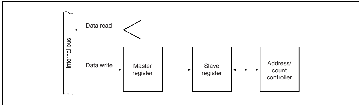
Figure 19-8. Buffer Register Configuration
