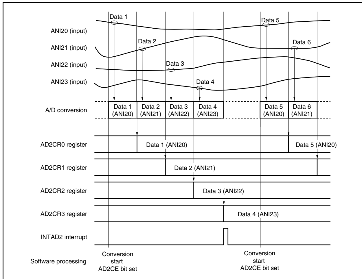
Figure 13-7. One-Shot Scan Mode Operation Timing
