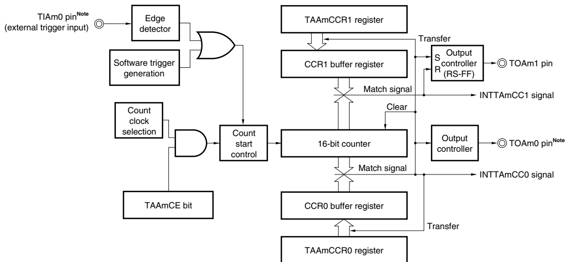
Figure 6-24. Configuration in External Trigger Pulse Output Mode
