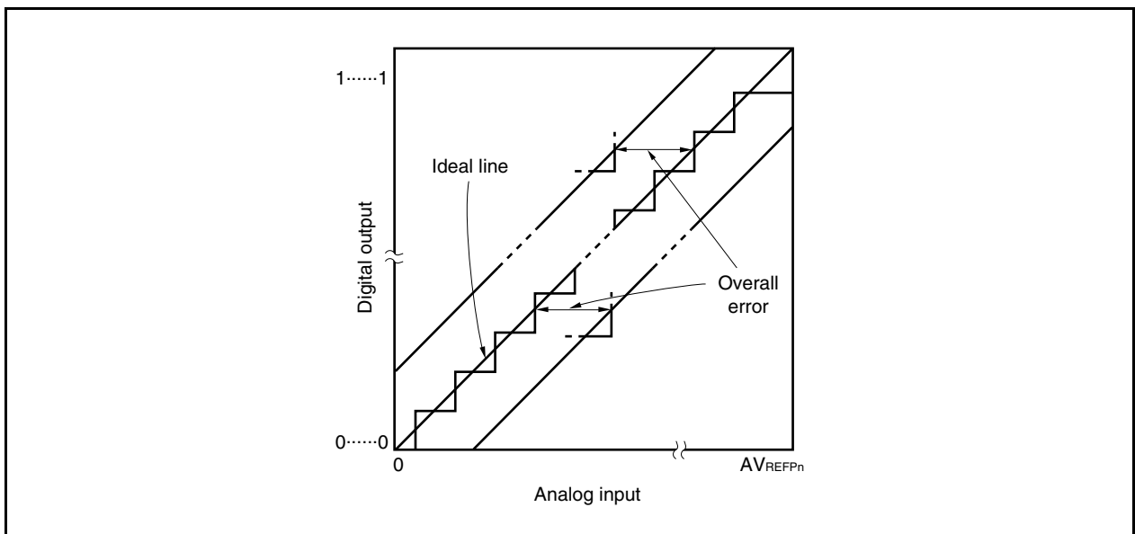
Figure 12-23. Overall Error
