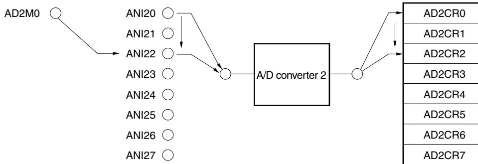
Figure 13-11. Operation Example of Software Trigger One-Shot Scan Mode: V850E/IG3
