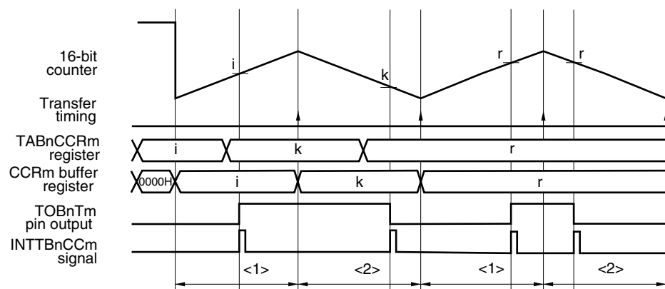
Figure 10-30. Example of Rewriting TABnCCRm Register
