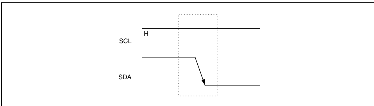
Figure 17-6. Start Conditions
