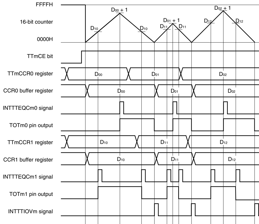
Figure 8-44. Basic Timing in Triangular-Wave PWM Output Mode
