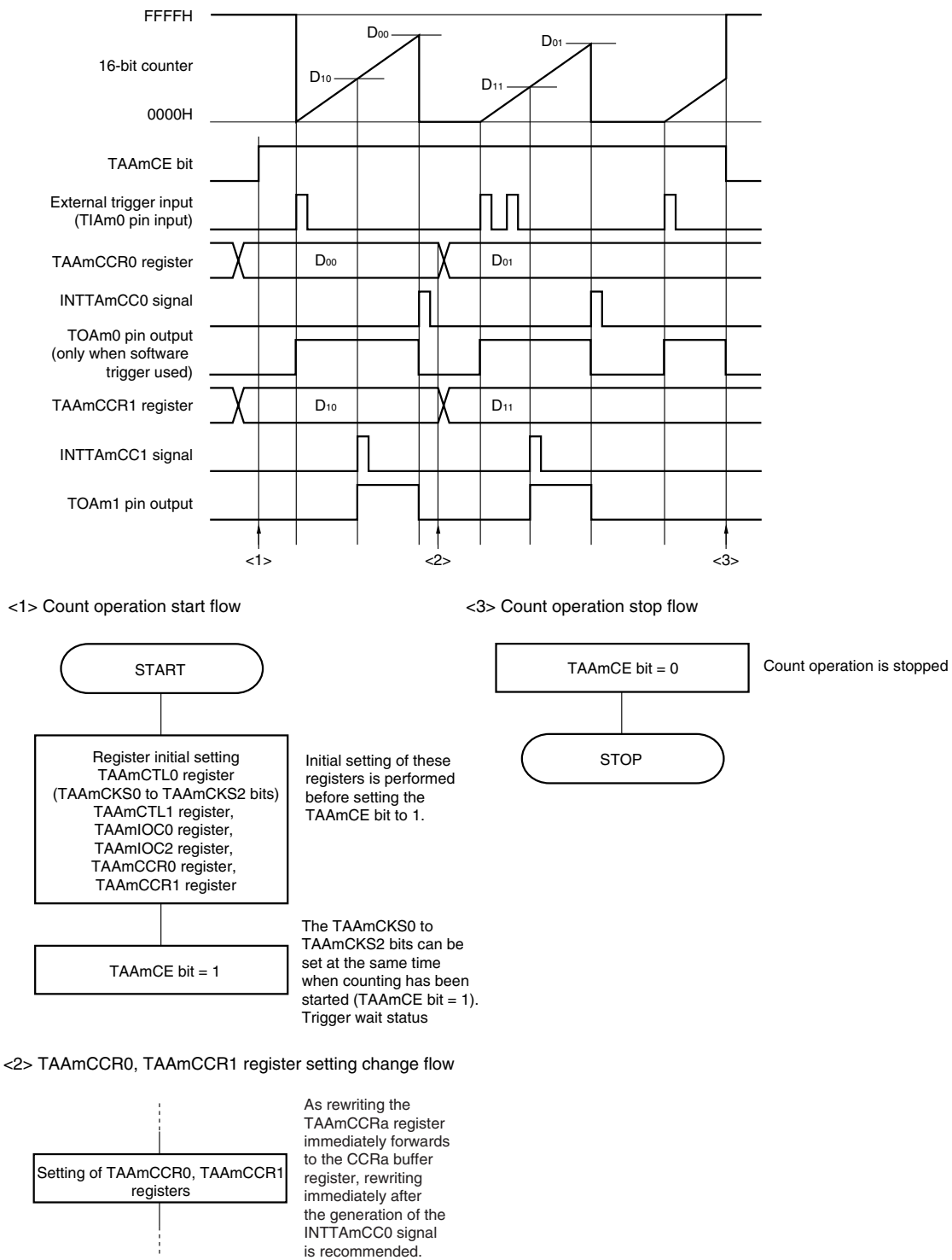
Figure 6-31. Software Processing Flow in One-Shot Pulse Output Mode
