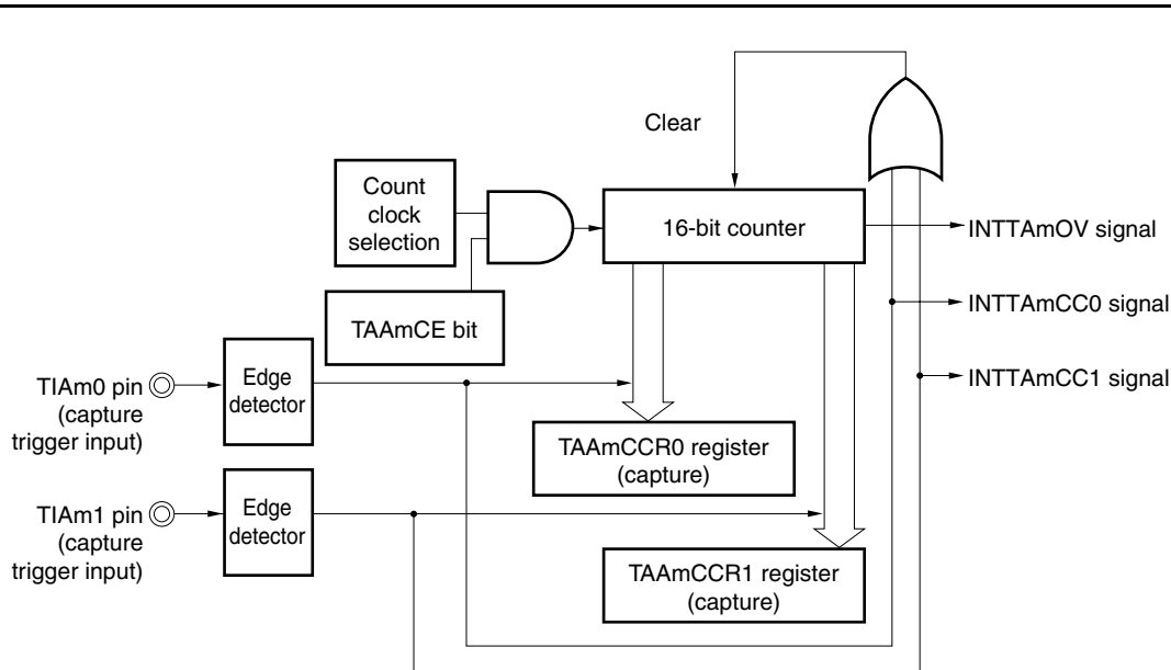
Figure 6-42. Configuration in Pulse Width Measurement Mode
