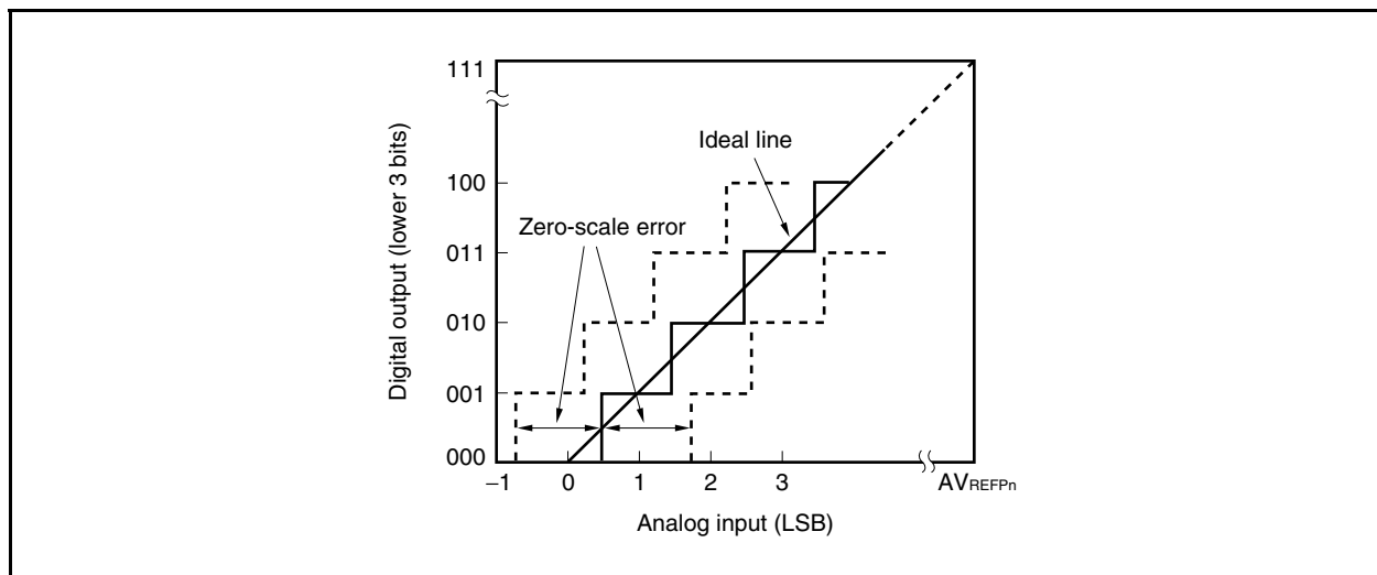
Figure 12-25. Zero-Scale Error
