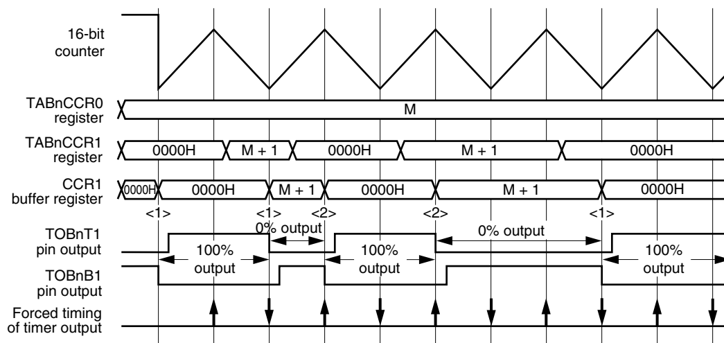
Figure 10-11. PWM Output Waveform from 0% to 100% and from 100% to 0% (With Dead Time)
