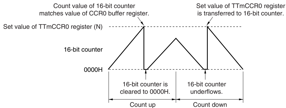
Figure 8-53. Operation Example (Count Operation in Range from 0000H to Set Value of TTmCCR0 Register)
