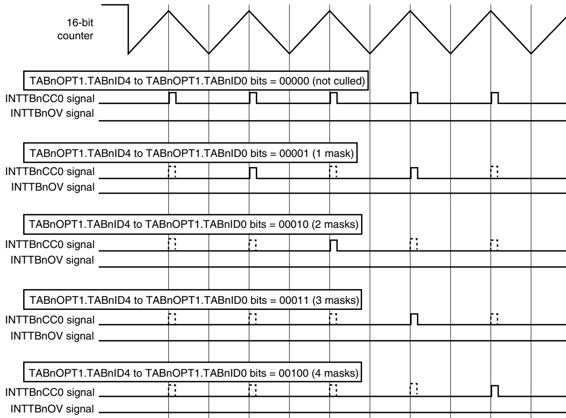
Figure 10-16. Interrupt Culling Operation When TABnOPT1.TABnICE Bit = 1, TABnOPT1.TABnIOE Bit = 0, TABnOPT2.TABnRDE Bit = 1 (Crest Interrupt Output)
