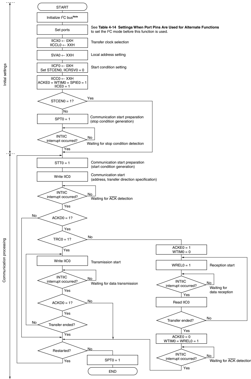
Figure 17-16. Master Operation in Single Master System
