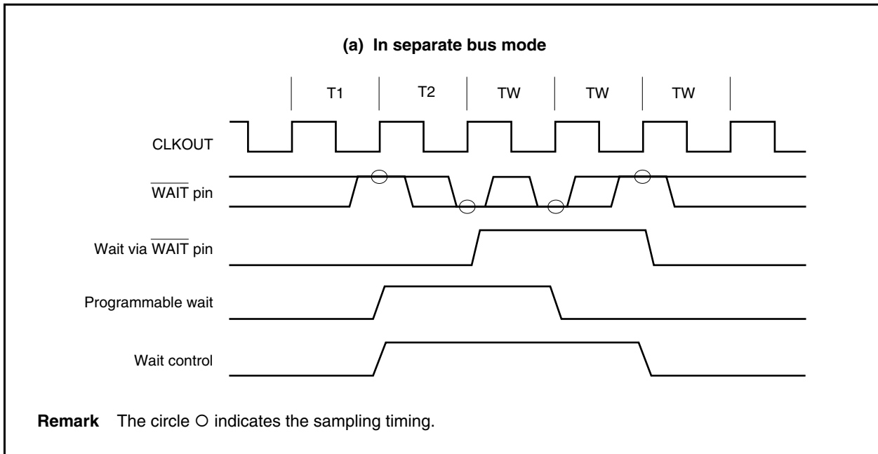
Figure 18-1. Example of Inserting Wait States (1/2)
