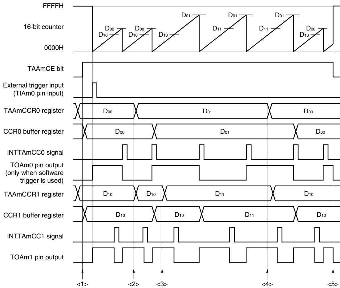
Figure 6-27. Software Processing Flow in External Trigger Pulse Output Mode (1/2)
