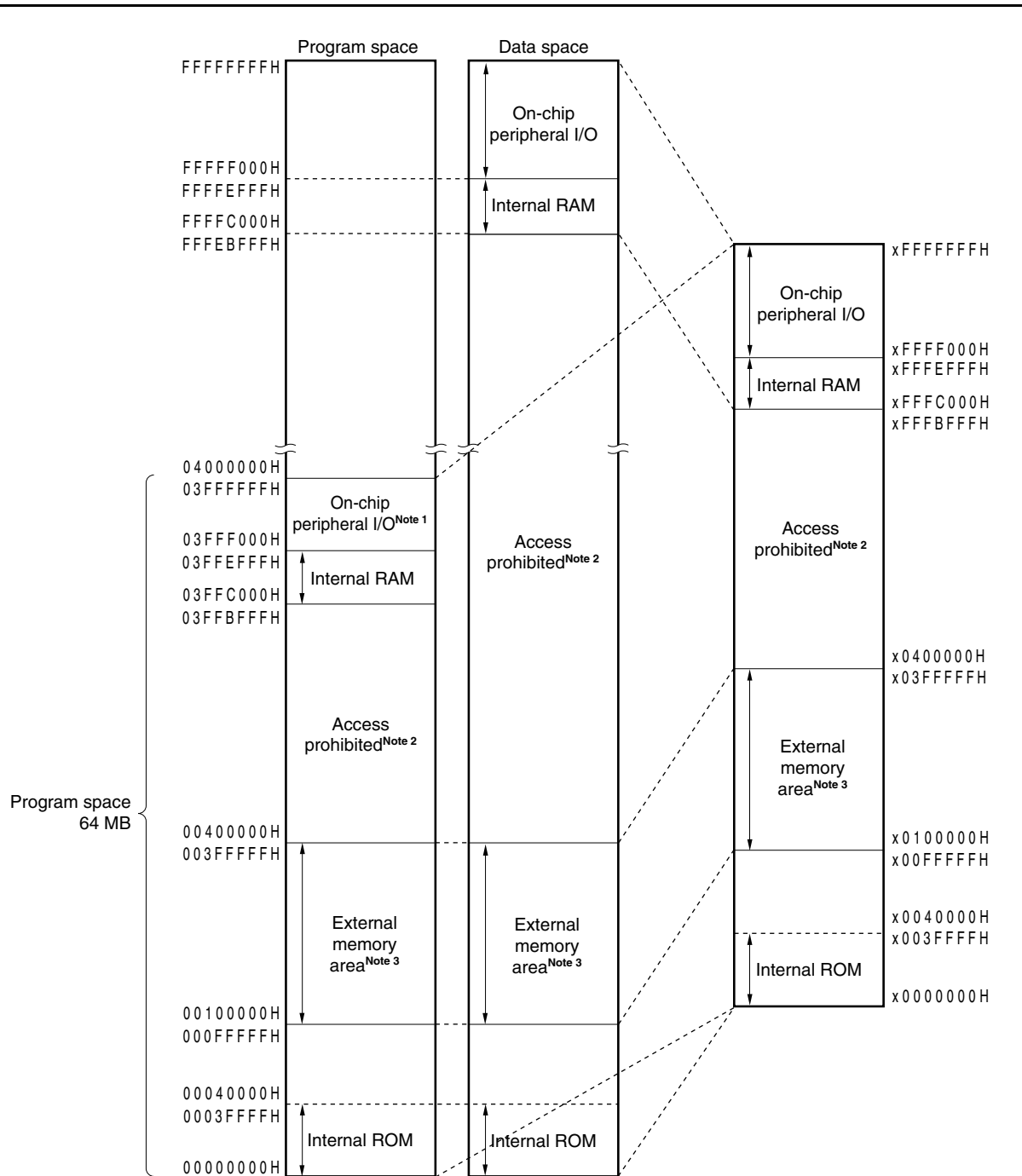
Figure 3-10. Recommended Memory Map
