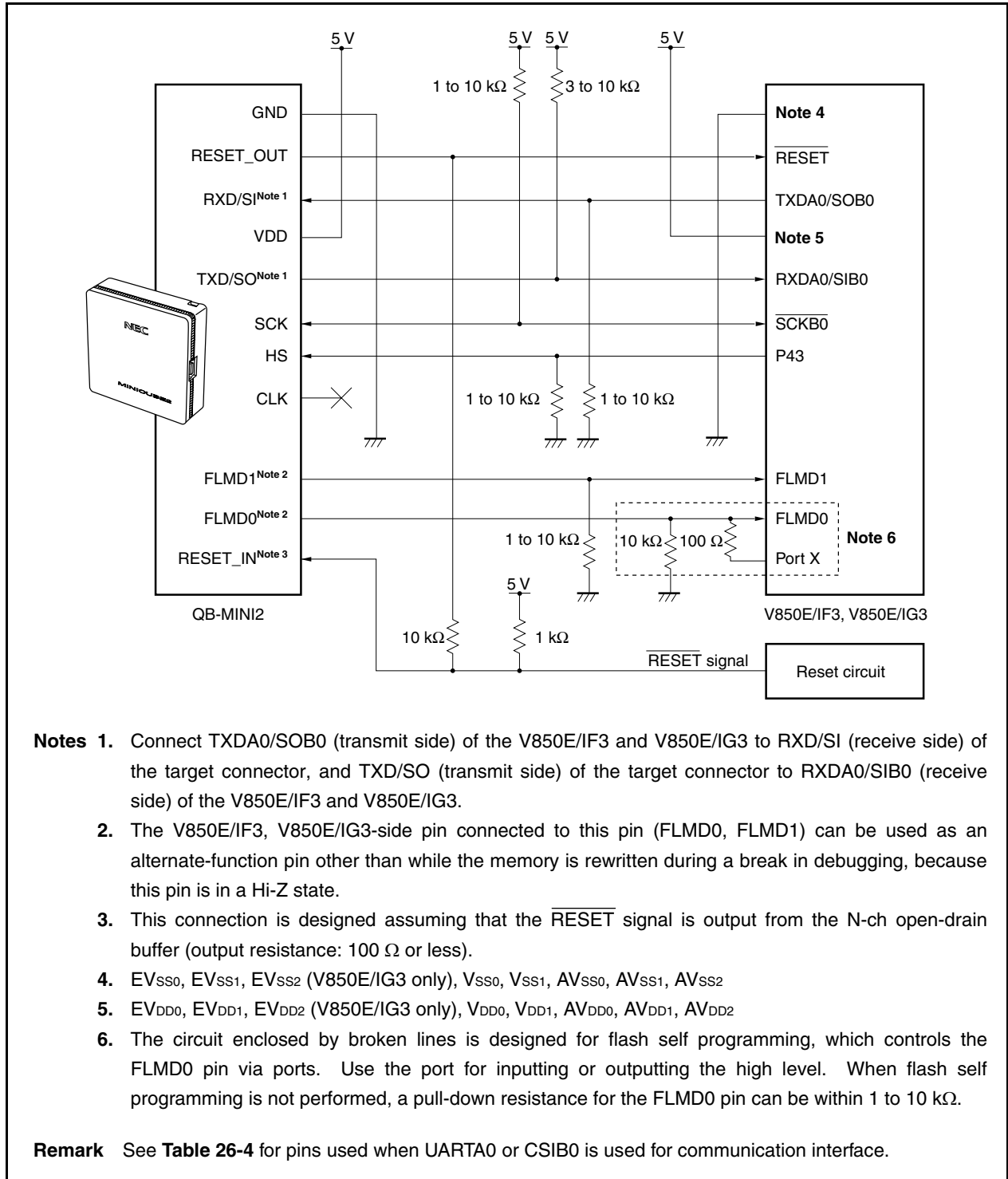
Figure 26-4. Circuit Connection Example When UARTA0/CSIB0 Is Used for Communication Interface
