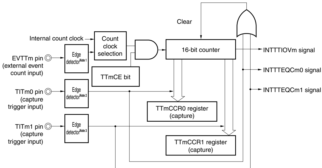
Figure 8-39. Configuration in Pulse Width Measurement Mode
