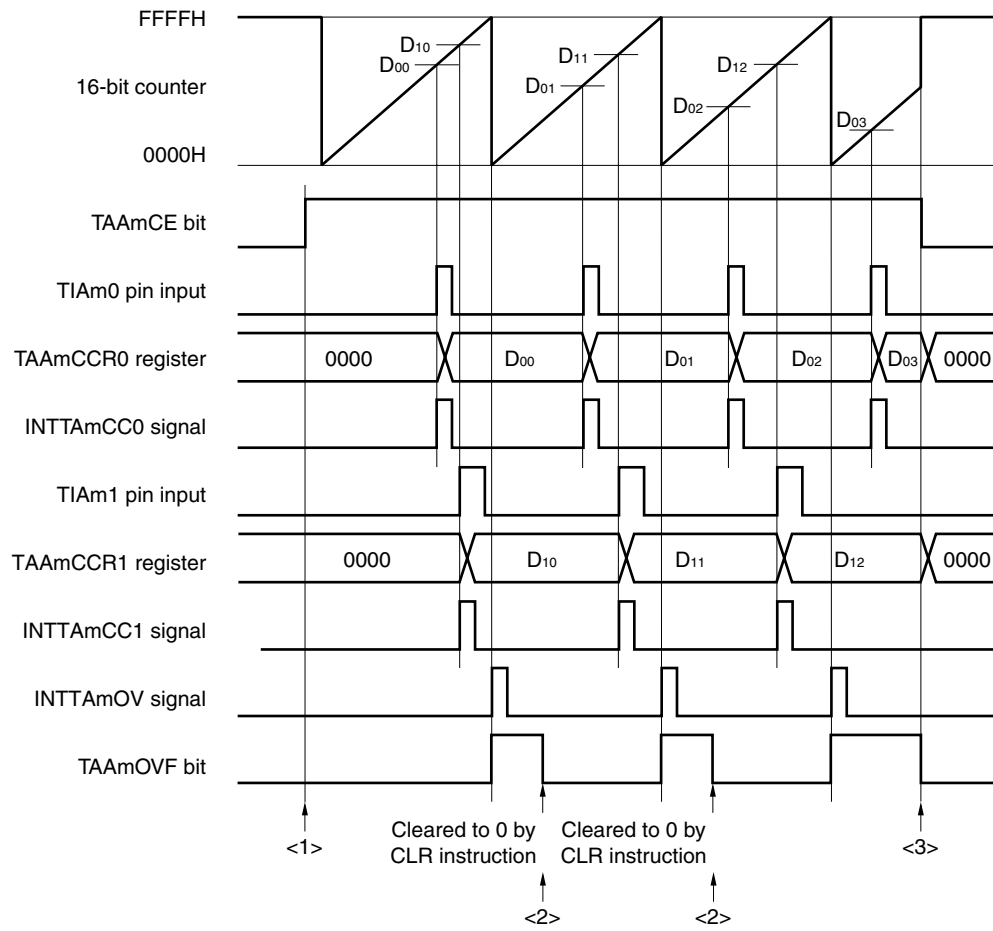
Figure 6-41. Software Processing Flow in Free-Running Timer Mode (Capture Function) (1/2)
