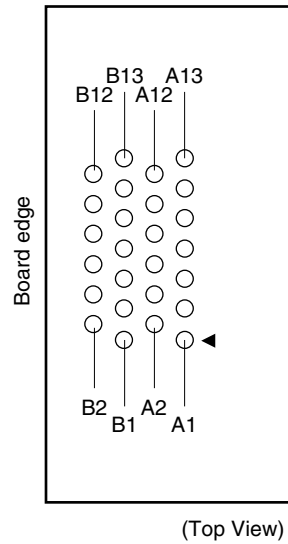
Figure 26-2. Pin Configuration of Emulator Connector (on Target System Side)
