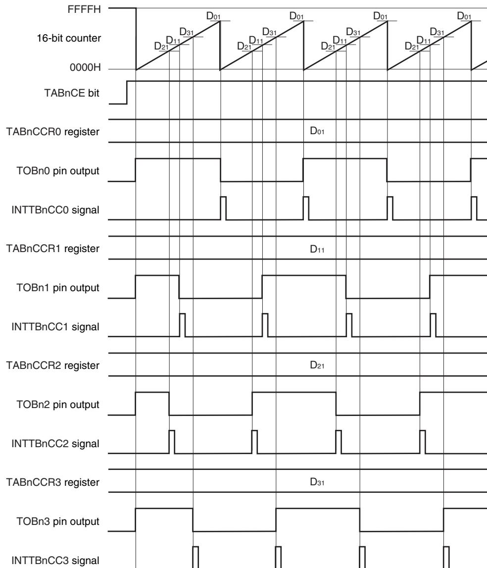
Figure 7-11. Timing Chart When D_{01} \geq D_{b1}
