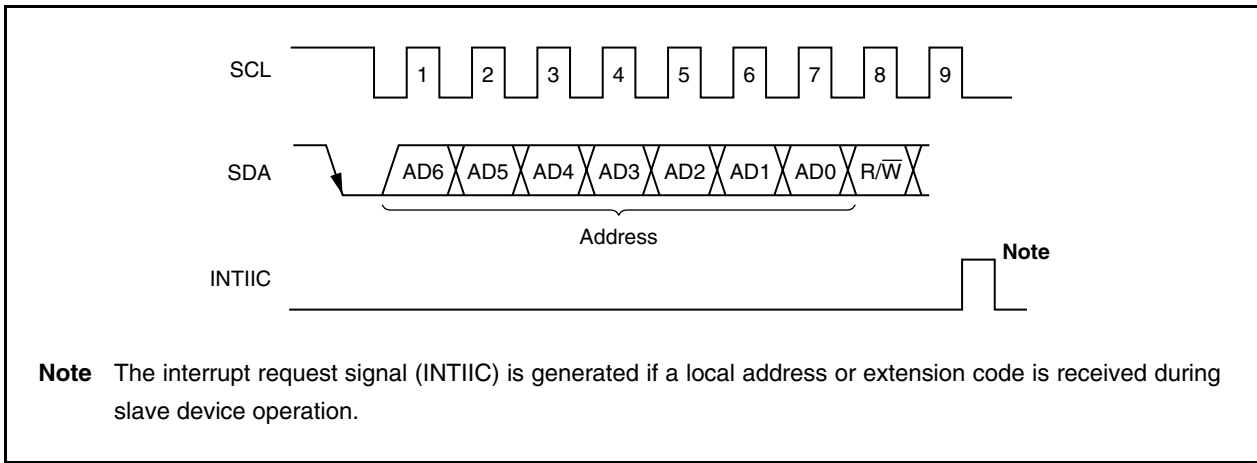
Figure 17-7. Address
