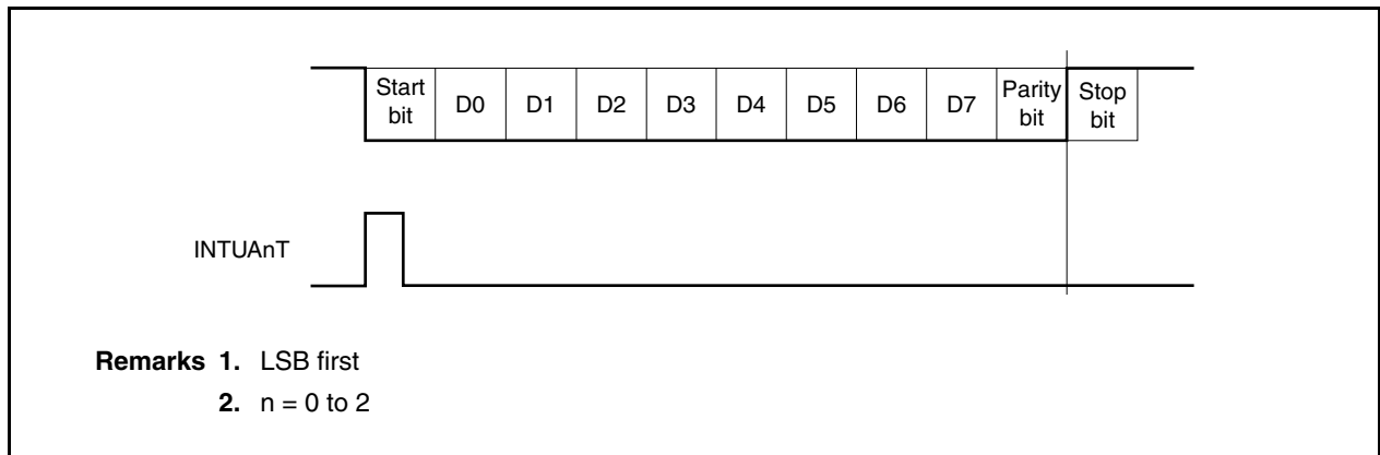
Figure 14-6. UART Transmission
