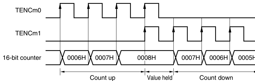
Figure 8-48. Operation Example (When Rising Edge Is Specified as Valid Edge of TENCm0 and TENCm1 Pins)
