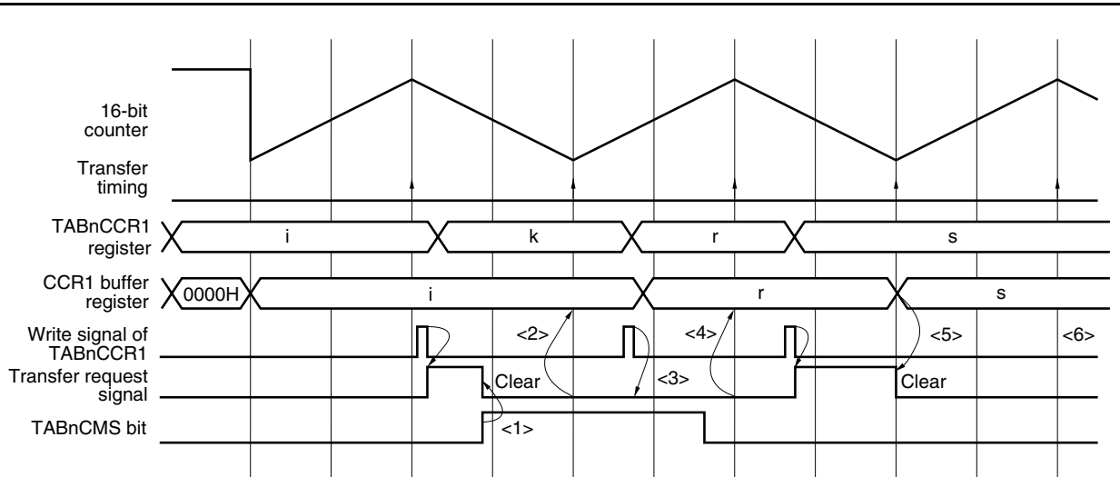
Figure 10-36. Rewriting TABnCMS Bit
