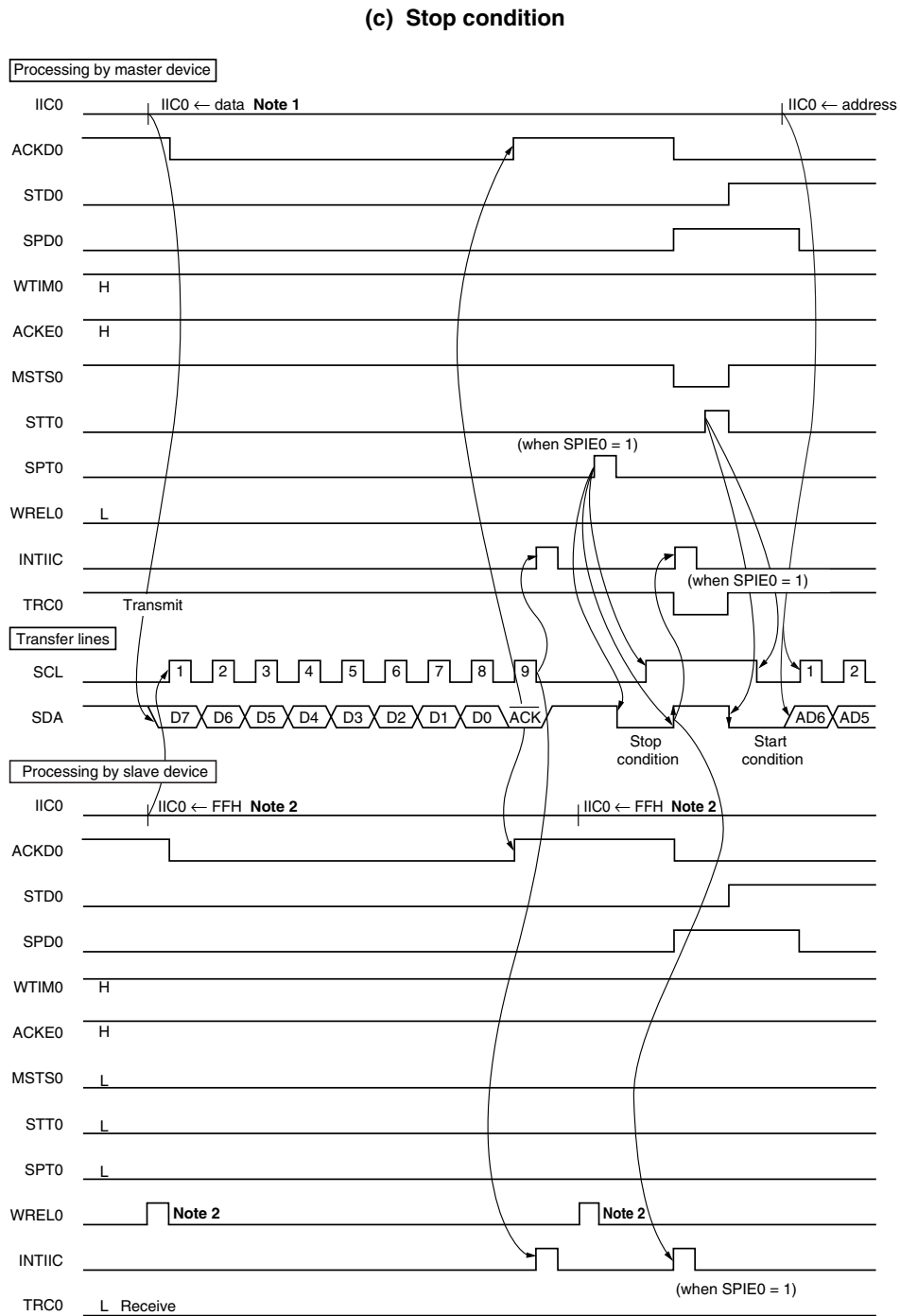
Figure 17-21. Example of Master to Slave Communication (When 9-Clock Wait Is Selected for Both Master and Slave) (3/3)
