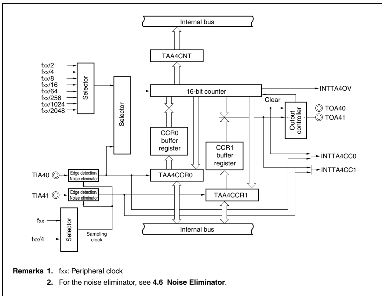
Figure 6-5. TAA4 Block Diagram
