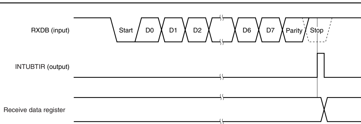
Figure 15-6. Timing of Asynchronous Serial Interface Reception End Interrupt Request Signal (INTUBTIR)
