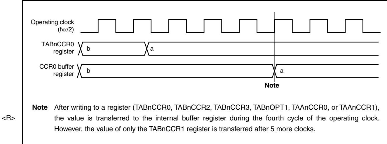
Figure 10-21. Timing of Reflecting Rewritten Value
