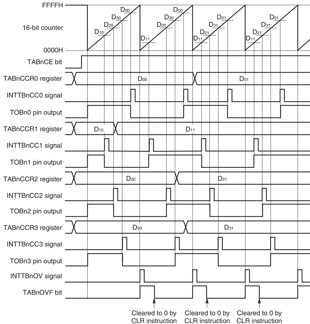
Figure 7-33. Basic Timing in Free-Running Timer Mode (Compare Function)
