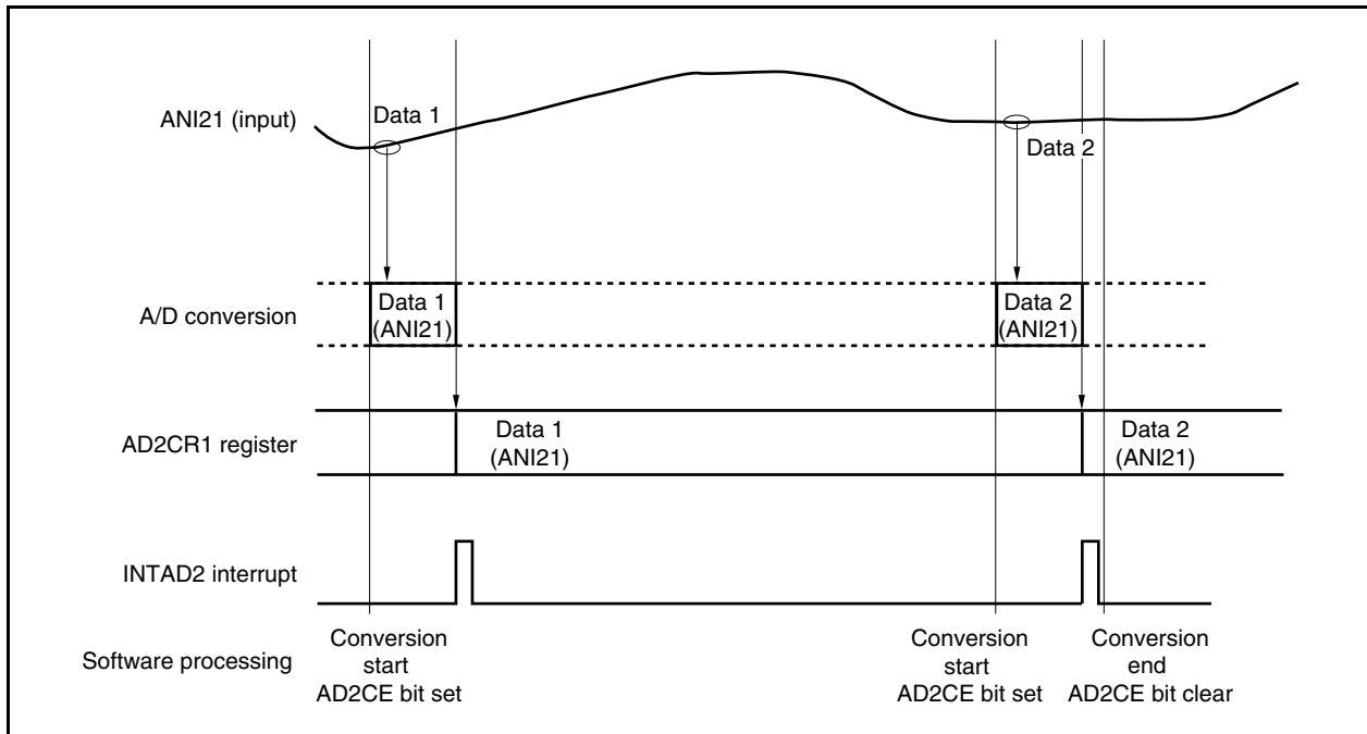
Figure 13-6. One-Shot Select Mode Operation Timing
