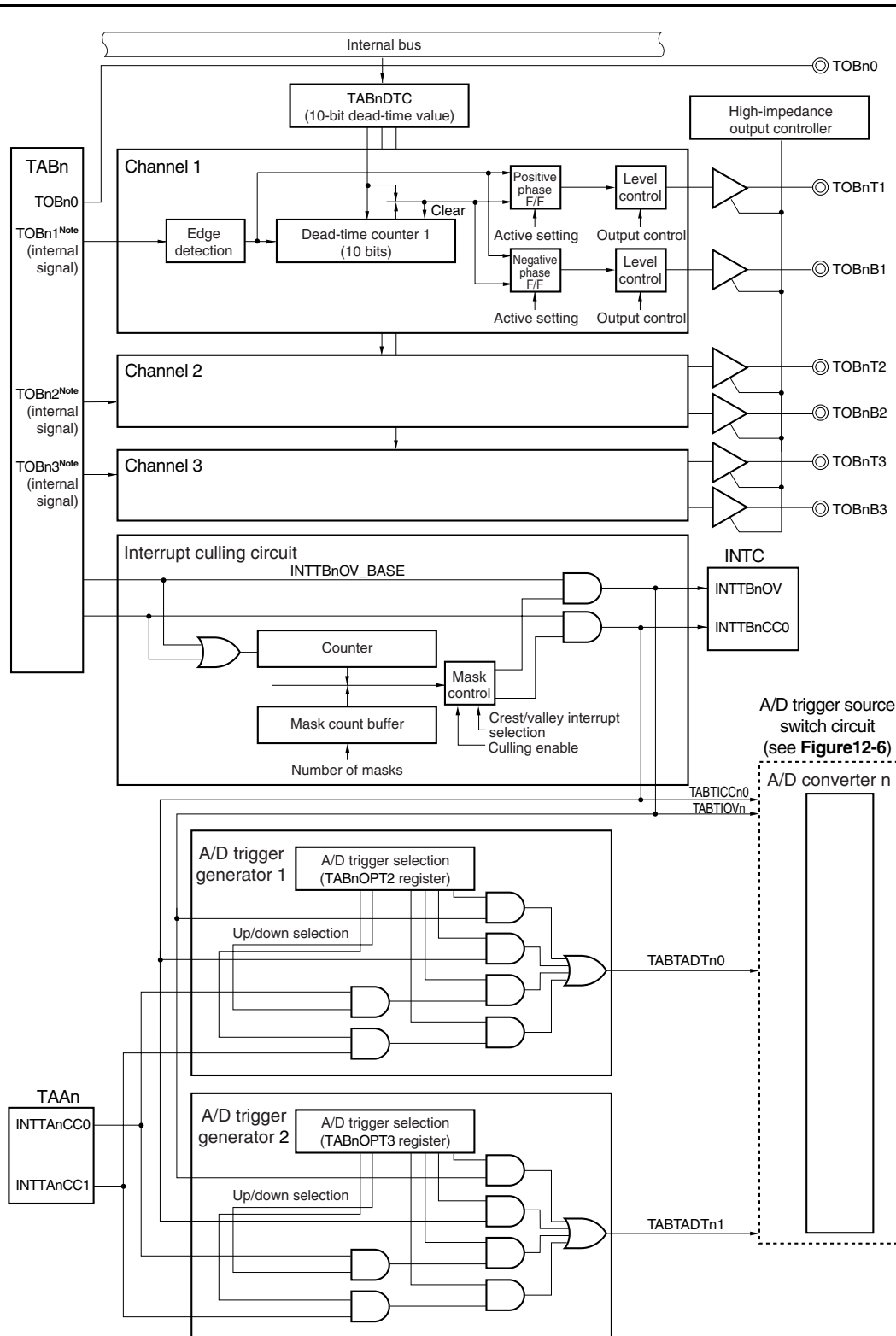
Figure 10-2. TMQn Option
