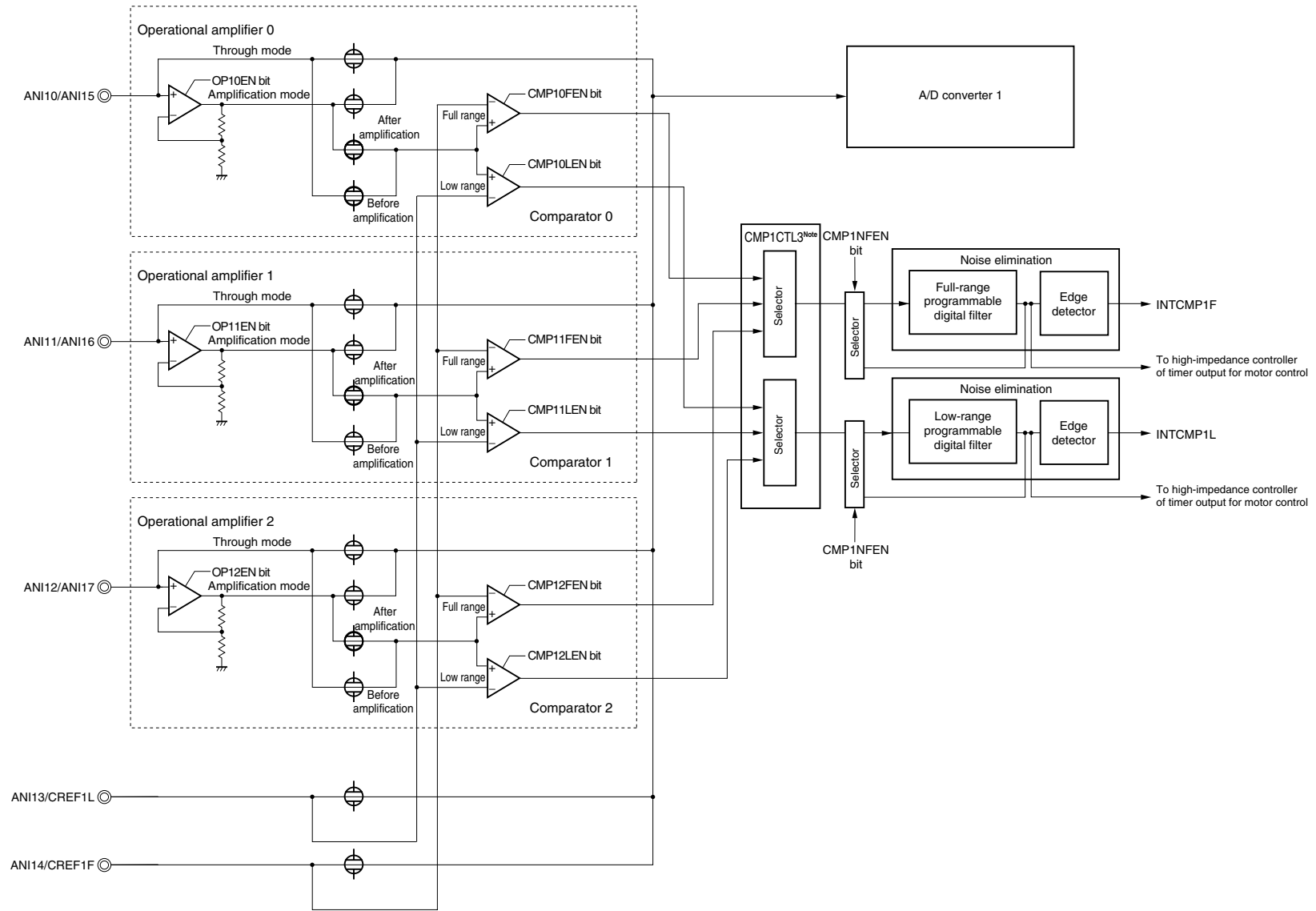
<R> Figure 12-4. Block Diagram of Operational Amplifier for Input Level Amplification and Overvoltage Detection Comparator in A/D Converter 1
