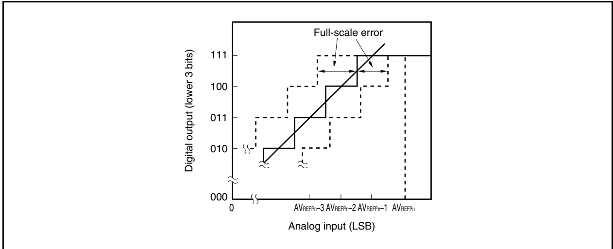
Figure 12-26. Full-Scale Error
