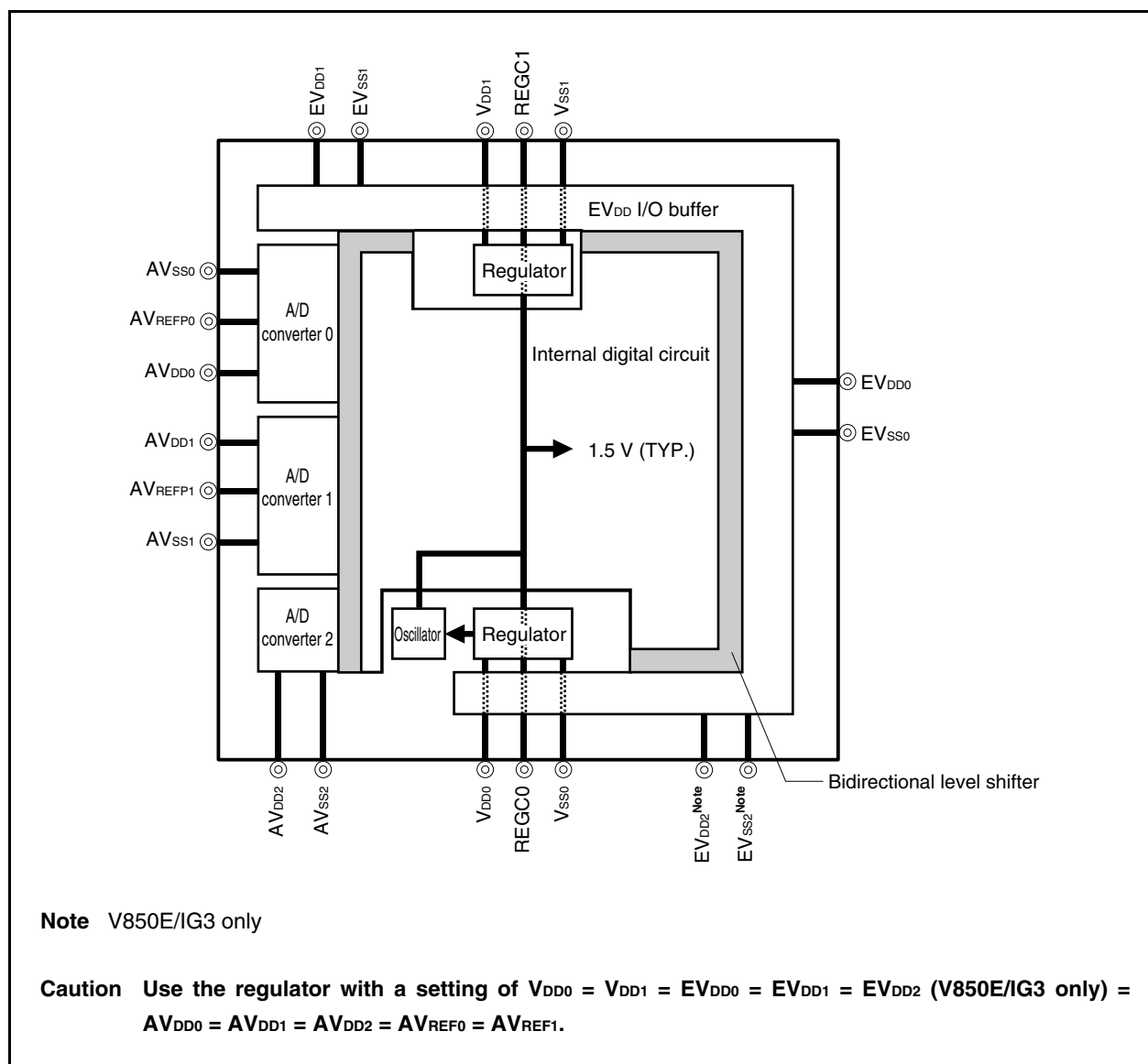
Figure 25-1. Regulator
