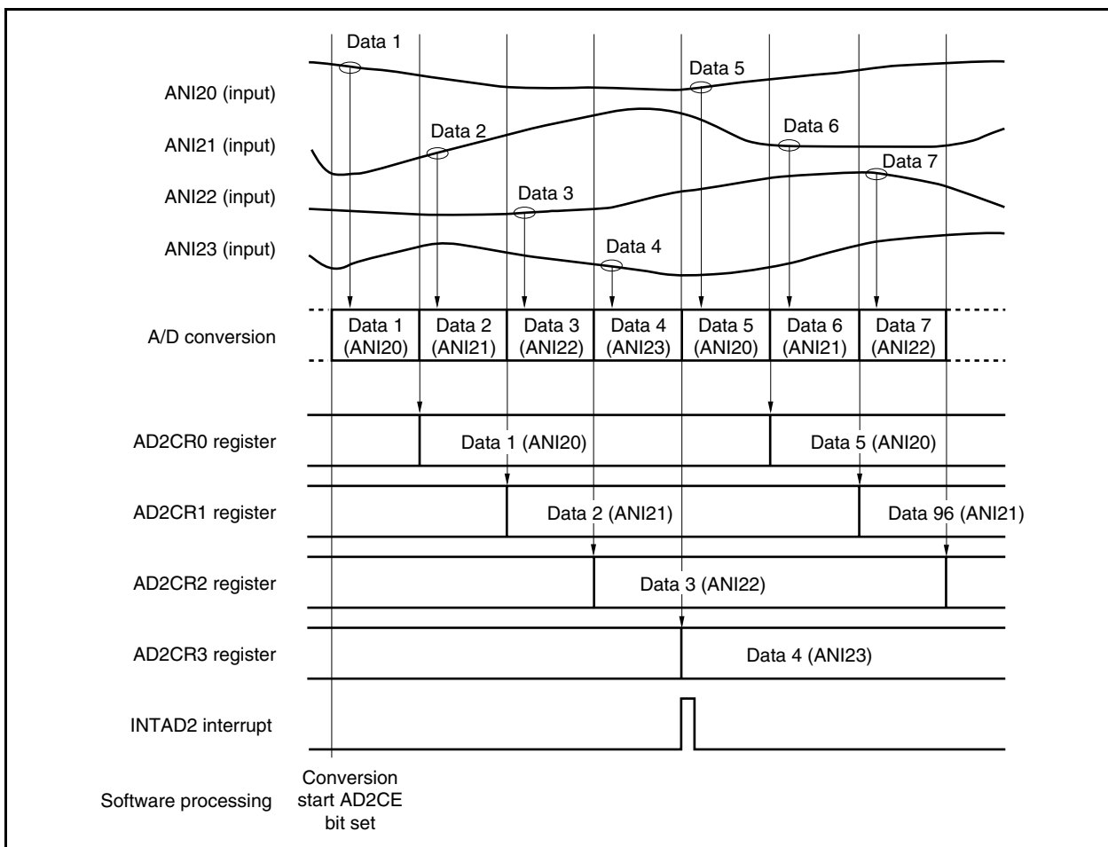
Figure 13-5. Continuous Scan Mode Operation Timing (When AD2M0.AD2MD1 and AD2M0.AD2MD0 Bits = 01, AD2S.AD2S2 to AD2S.AD2S0 Bits = 011): V850E/IG3
