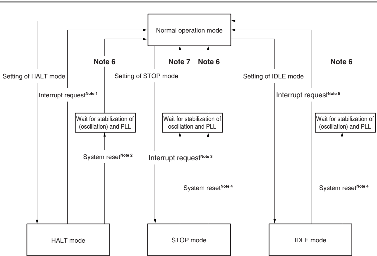
Figure 21-1. Status Transition
