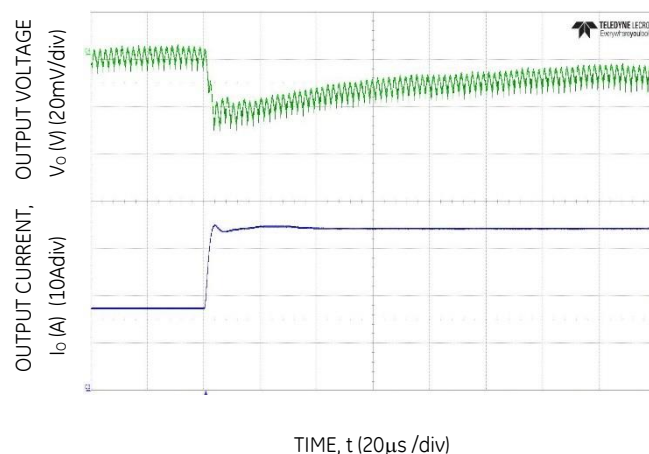
Figure 10. Transient Response to Dynamic Load Change from 50% to 100% at 12Vin, C_{out}=8\times 47\mu\text{F}+14\times 330\mu\text{F} , C_{Tune}=10\text{nF} , R_{Tune}=300\Omega
