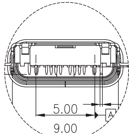
DETAIL 2 SCALE 2:1
