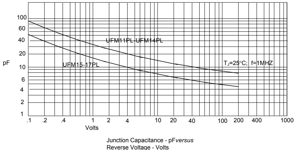
Figure 4 Junction Capacitance
