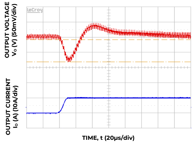
Figure 28 Transient Response to Dynamic Load Change from 50% to 100% at 12V in , C out = 5x47µF +1x330µF, C Tune =2200pF & R Tune =220 ohms
