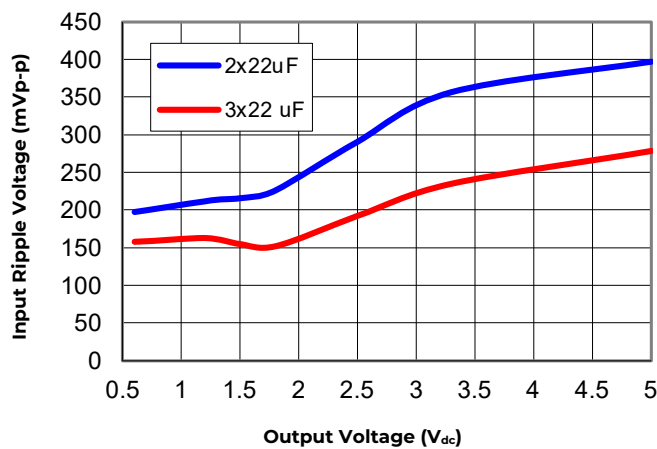
Figure 37. Input ripple voltage for various output voltages with 2x22 μF or 3x22 μF ceramic capacitors at the input (20A load). Input voltage is 12V.
