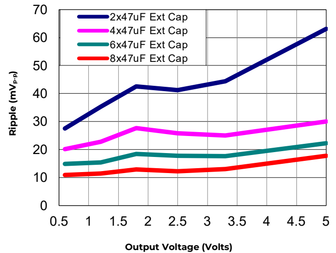
Figure 38. Output ripple voltage for various output voltages with external 2x47 μF, 4x47 μF or 6x47 μF ceramic capacitors at the output (20A load). Input voltage is 12V.
