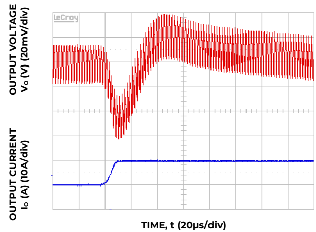
Figure 22. Transient Response to Dynamic Load Change from 50% to 100% at 12V in , C out = 2x47µF +2x330µF, C Tune =3300pF & R Tune =220 ohms
