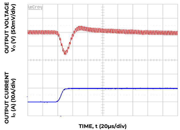
Figure 34. Transient Response to Dynamic Load Change from 50% to 100% at 12V in , C out = 8x47µF, C Tune =1500pF & R Tune =220 ohms
