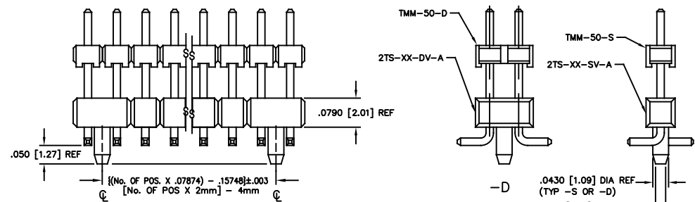
FIG 3 (-A MOLDED ALIGNMENT PIN OPTION) SAME AS FIG 1 EXCEPT WHERE NOTED.
