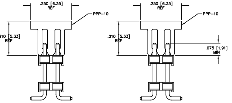
FIG 5 (-M OPTION) (SEE NOTE 10)
