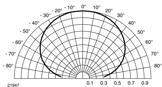
Fig. 9 - Horizontal Directivity
