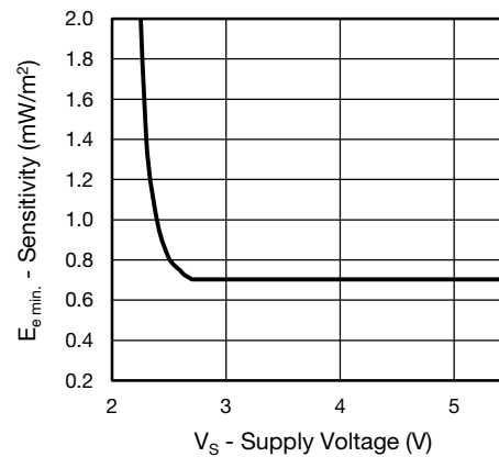
Fig. 8 - Sensitivity vs. Supply Voltage
