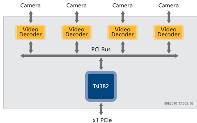
Figure 2 DVR Application
