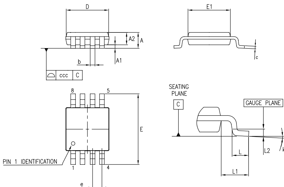
Figure 47. MiniSO8 package outline
