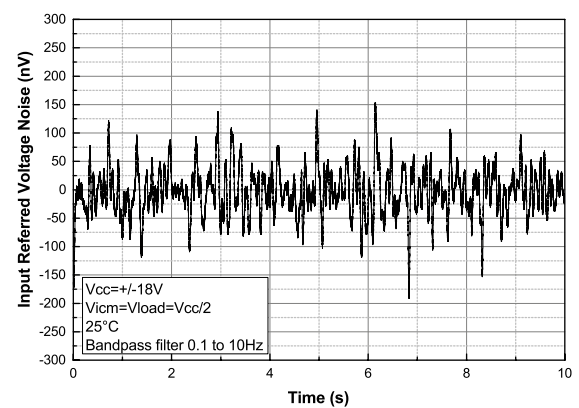
Figure 36. Noise vs. time at V_{CC} = 36\text{ V}
