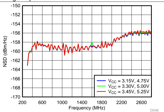
Figure 33. Noise vs Supply, Typical Operating Mode
