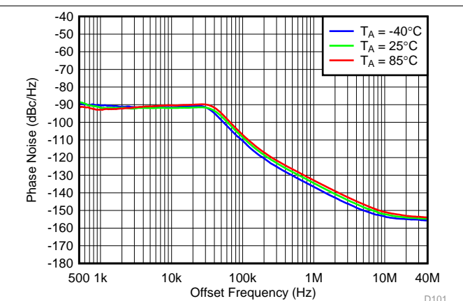
Figure 89. 2700 MHz Frac-N (Closed Loop Phase Noise) vs Temperature
