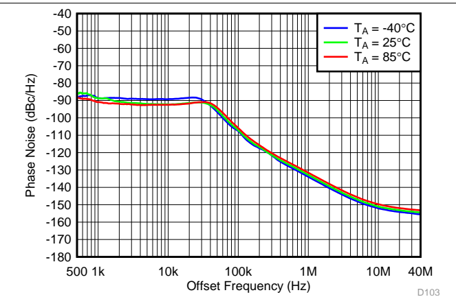
Figure 91. 3600 MHz Frac-N (Closed Loop Phase Noise) vs Temperature
