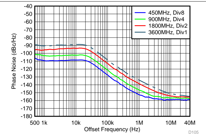
Figure 93. 450, 900, 1800, 3600 MHz Closed Loop Phase Noise vs Offset Frequency
