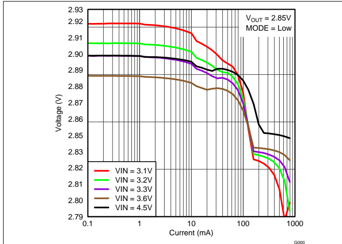
Figure 19. TPS82693 DC Output Voltage vs Load Current
