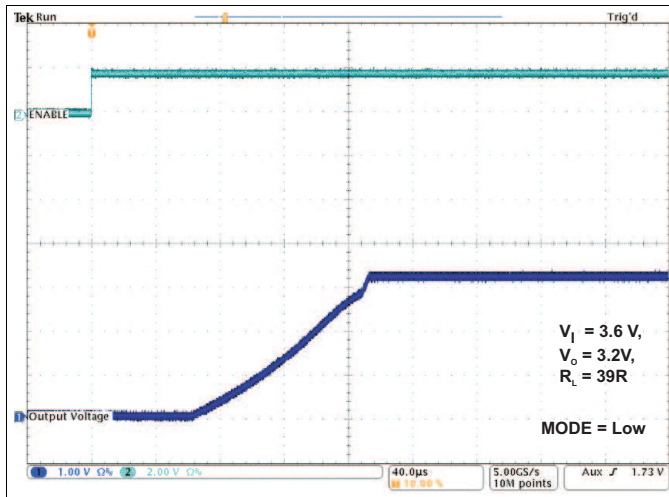
Figure 25. TPS82699 Start-Up
