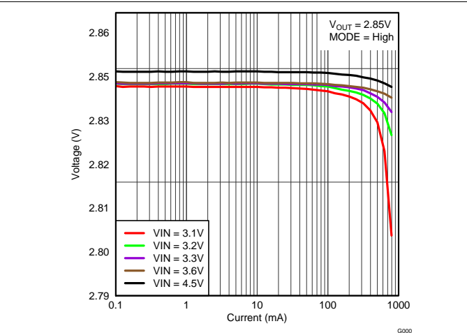
Figure 20. TPS82693dc Output Voltage vs Load Current
