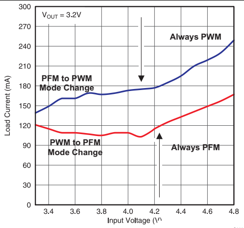
Figure 21. TPS82699 PFM/PWM Boundaries
