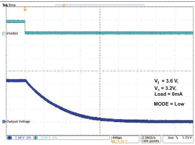
Figure 26. TPS82699 Shut-Down
