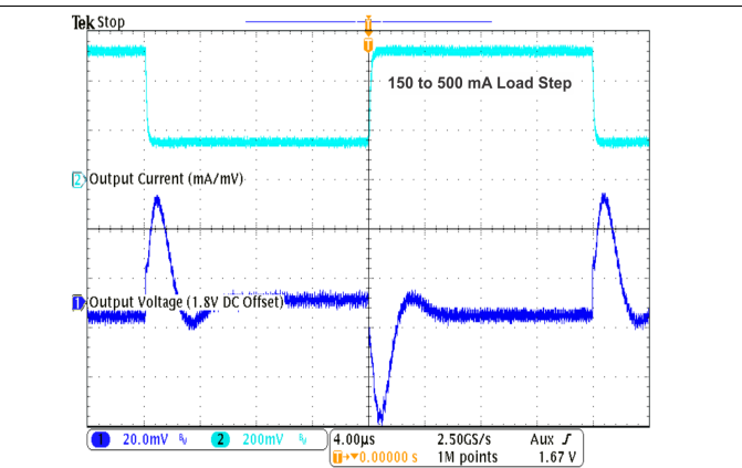
Figure 24. Load Transient Response in PFM/PWM Operation
