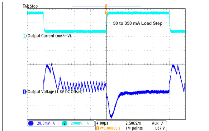
Figure 23. Load Transient Response in PFM/PWM Operation
