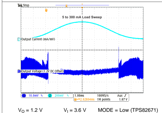
Figure 37. AC Load Transient Response
