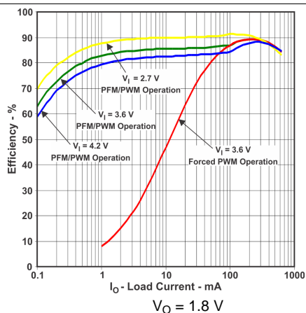
Figure 11. Efficiency vs. Load Current
