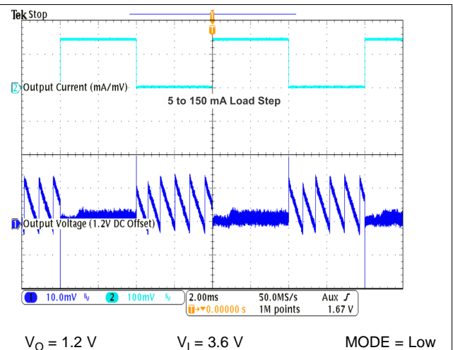
Figure 30. Load Transient Response in PFM/PWM Operation
