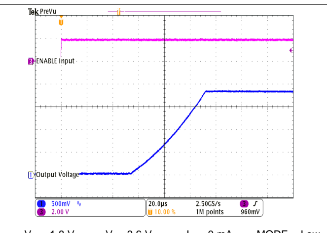
Figure 40. Start-Up
