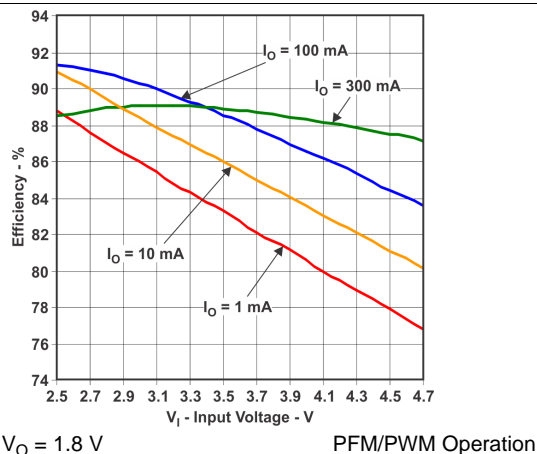
Figure 13. Efficiency vs. Input Voltage
