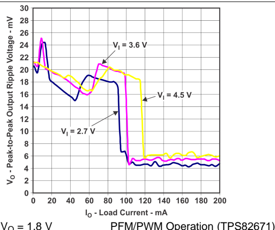
Figure 14. Peak-to-Peak Output Ripple Voltage vs. Load Current
