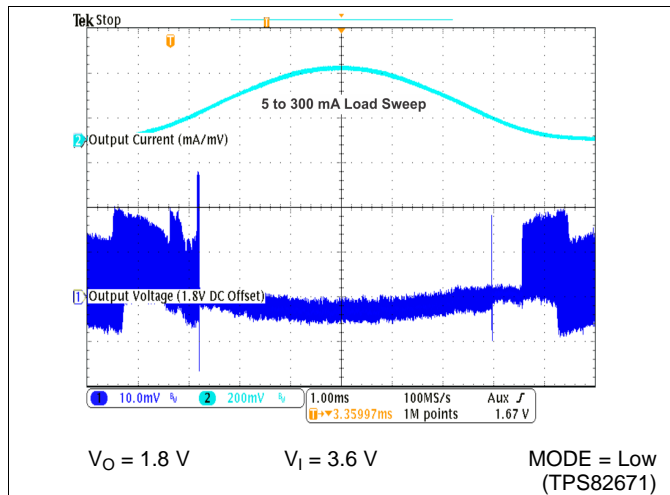
Figure 29. AC Load Transient Response
