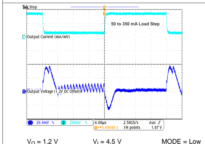
Figure 33. Load Transient Response in PFM/PWM Operation
