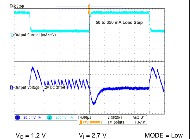
Figure 32. Load Transient Response in PFM/PWM Operation
