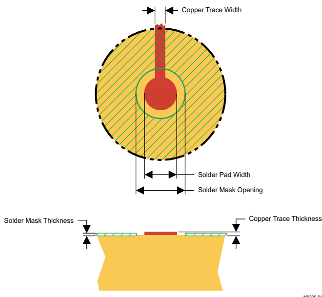
Figure 42. Recommended Land Pattern Image And Dimensions
