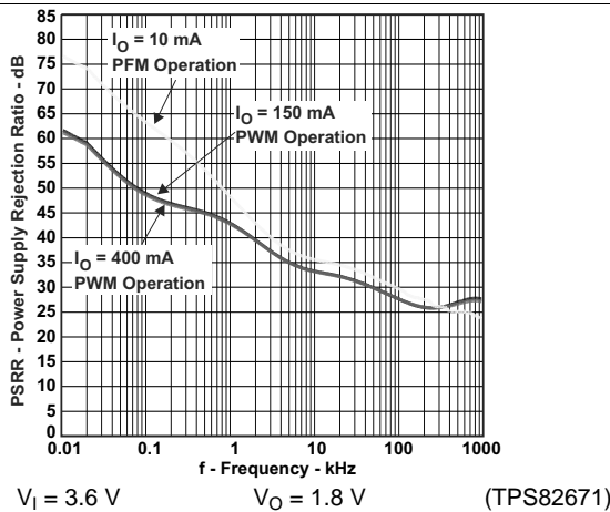
Figure 3. Power Supply Rejection Ratio vs. Frequency
