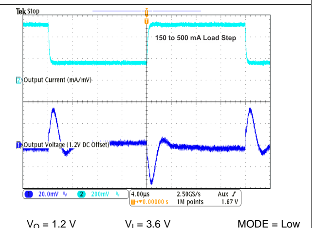
Figure 34. Load Transient Response in PFM/PWM Operation
