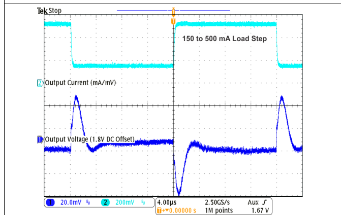
Figure 25. Load Transient Response in PFM/PWM Operation
