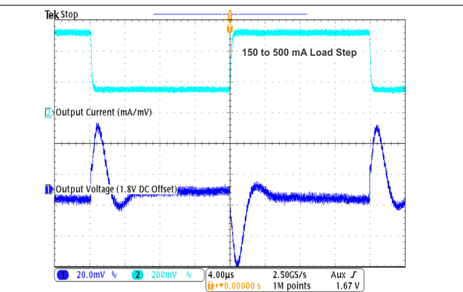
Figure 26. Load Transient Response in PFM/PWM Operation
