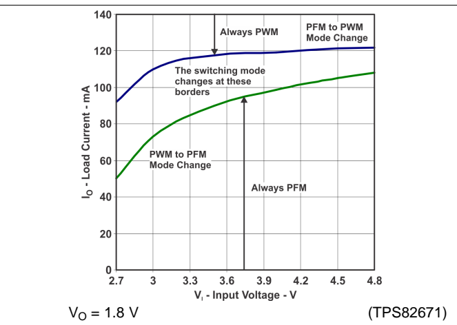
Figure 38. PFM/PWM Boundaries
