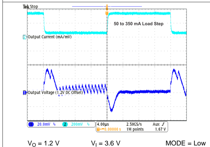
Figure 31. Load Transient Response in PFM/PWM Operation
