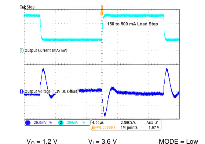
Figure 34. Load Transient Response in PFM/PWM Operation
