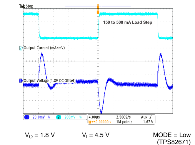
Figure 28. Load Transient Response in PFM/PWM Operation
