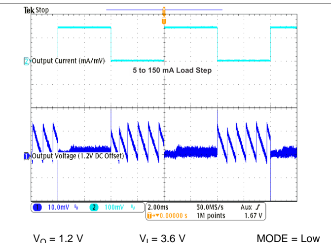
Figure 30. Load Transient Response in PFM/PWM Operation
