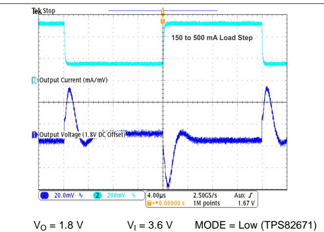
Figure 26. Load Transient Response in PFM/PWM Operation
