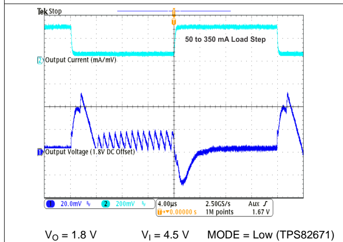
Figure 25. Load Transient Response in PFM/PWM Operation
