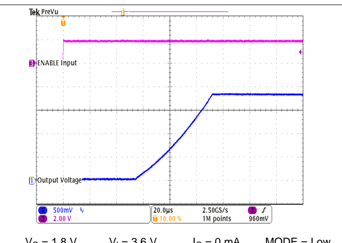
Figure 40. Start-Up
