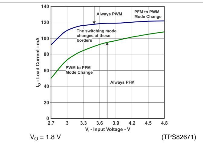
Figure 38. PFM/PWM Boundaries
