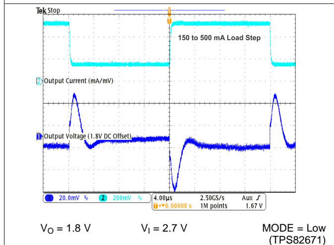
Figure 27. Load Transient Response in PFM/PWM Operation
