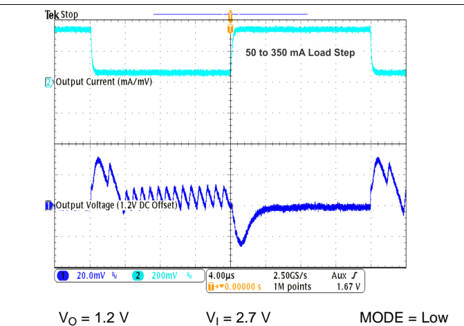
Figure 32. Load Transient Response in PFM/PWM Operation
