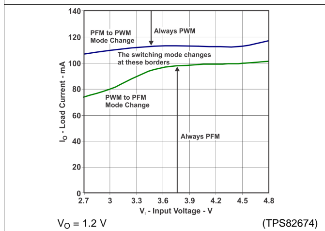
Figure 39. PFM/PWM Boundaries
