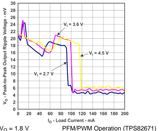
Figure 14. Peak-to-Peak Output Ripple Voltage vs. Load Current
