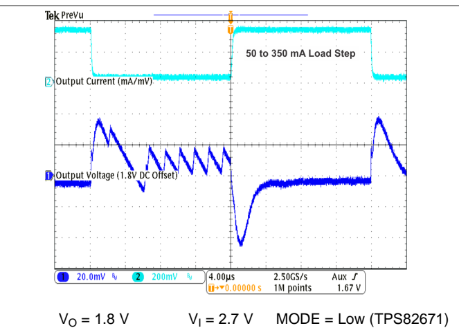
Figure 24. Load Transient Response in PFM/PWM Operation
