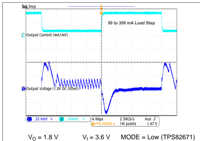
Figure 23. Load Transient Response in PFM/PWM Operation
