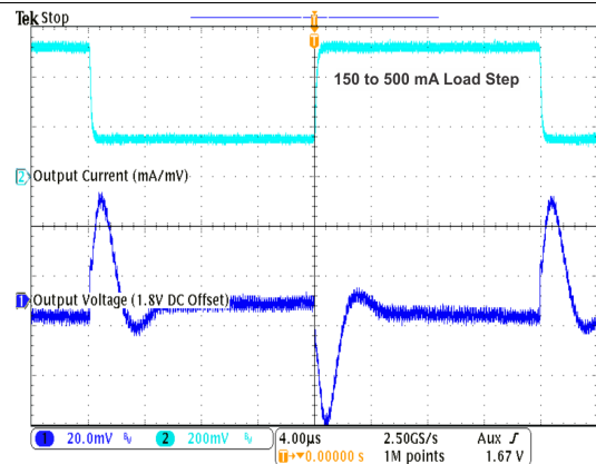
Figure 26. Load Transient Response in PFM/PWM Operation
