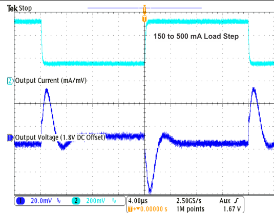
Figure 24. Load Transient Response in PFM/PWM Operation
