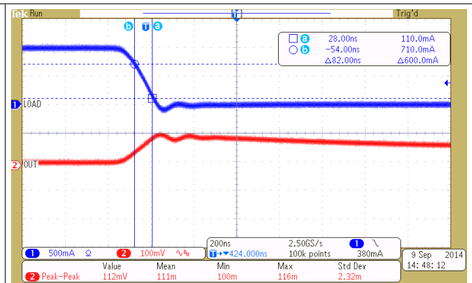
Figure 26. 1-A Load, Expanded View (High to Low), Slew Rate = 7.3 A/µS
