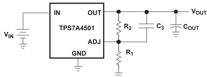
Figure 24. Compensation Schematic
