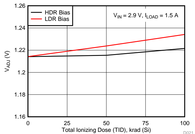
V_{ADJ} Radiation Drift Curve
