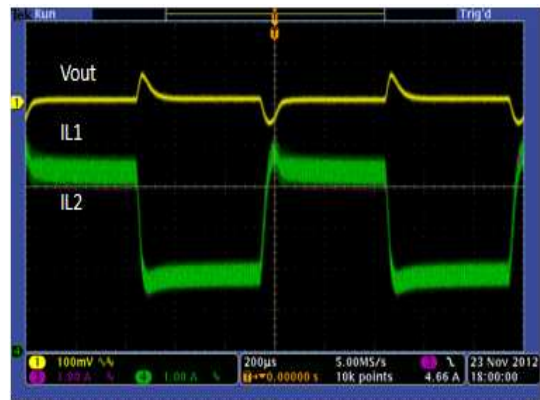
Figure 36. Load Transient, Current Share Mode Operation ( I_O = 4\text{ A} - 9\text{ A} )
