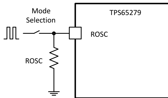
Figure 43. Resistor Mode and Synchronization Mode
