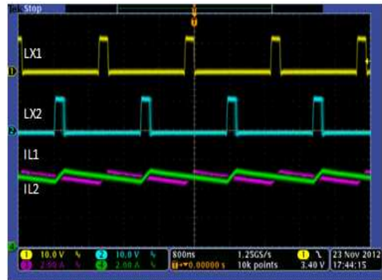
Figure 34. Steady State of Current Share Mode Operation ( I_O = 10\text{ A} )
