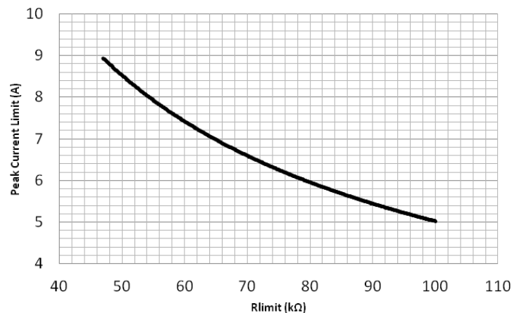
Figure 44. Peak Current Limit vs. R limit
