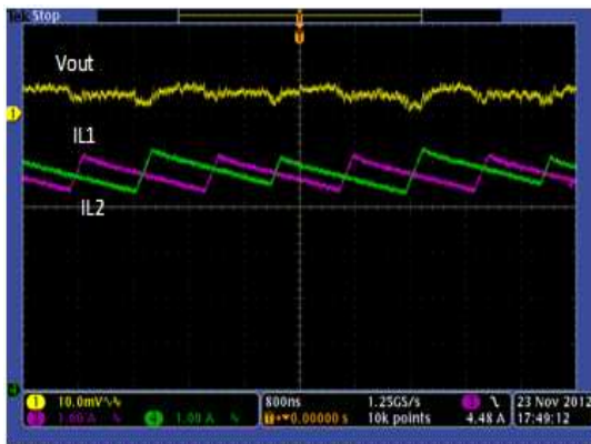
Figure 35. Output Ripple, Current Share Mode Operation ( I_O = 10\text{ A} )
