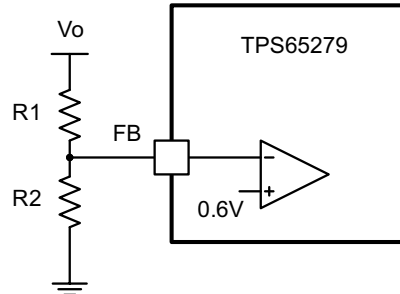
Figure 40. Voltage Divider Circuit
