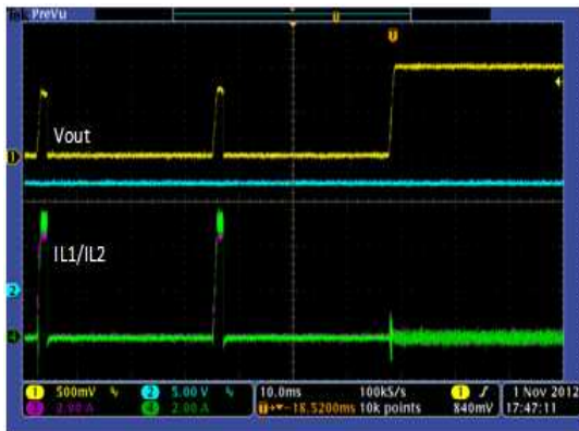
Figure 37. Hiccup Recover, Current Share Mode
