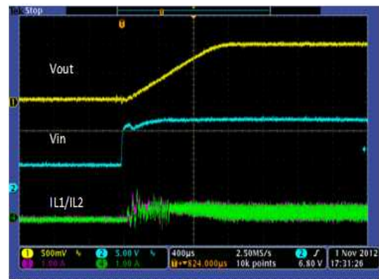
Figure 32. Current Share Mode Startup
