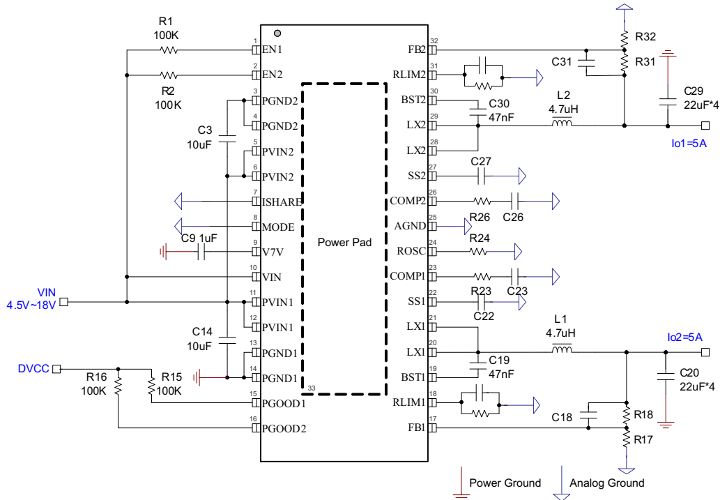
Figure 1. Dual Mode Operation to Deliver 5 A at Buck1 and 5 A at Buck2
