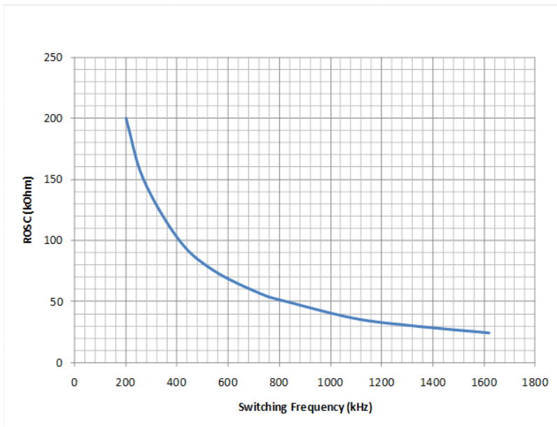
Figure 42. ROSC vs Switching Frequency
