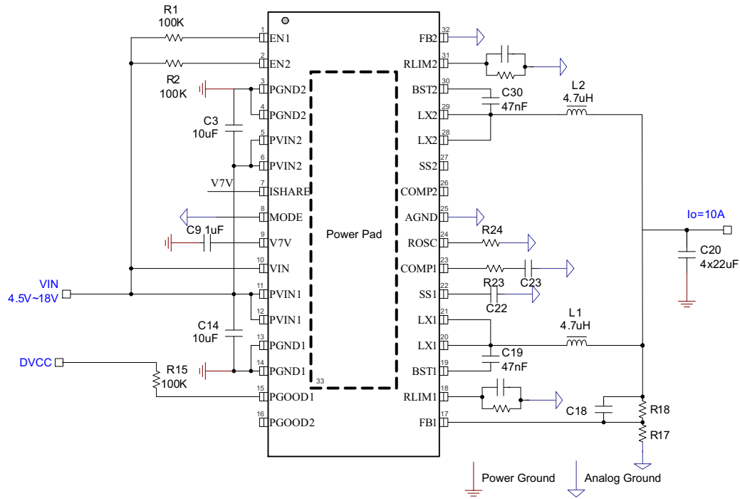
Figure 2. Share Mode Operation to Deliver 10 A
