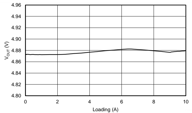
Figure 38. Current Share Mode, 5-V Load Regulation
