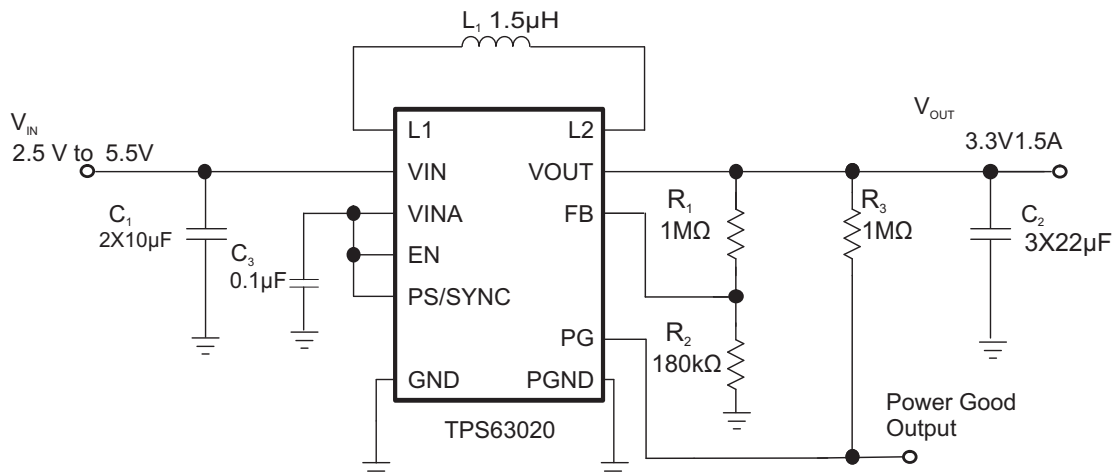
Figure 4. Application Circuit
