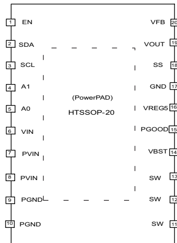
Terminal Functions
