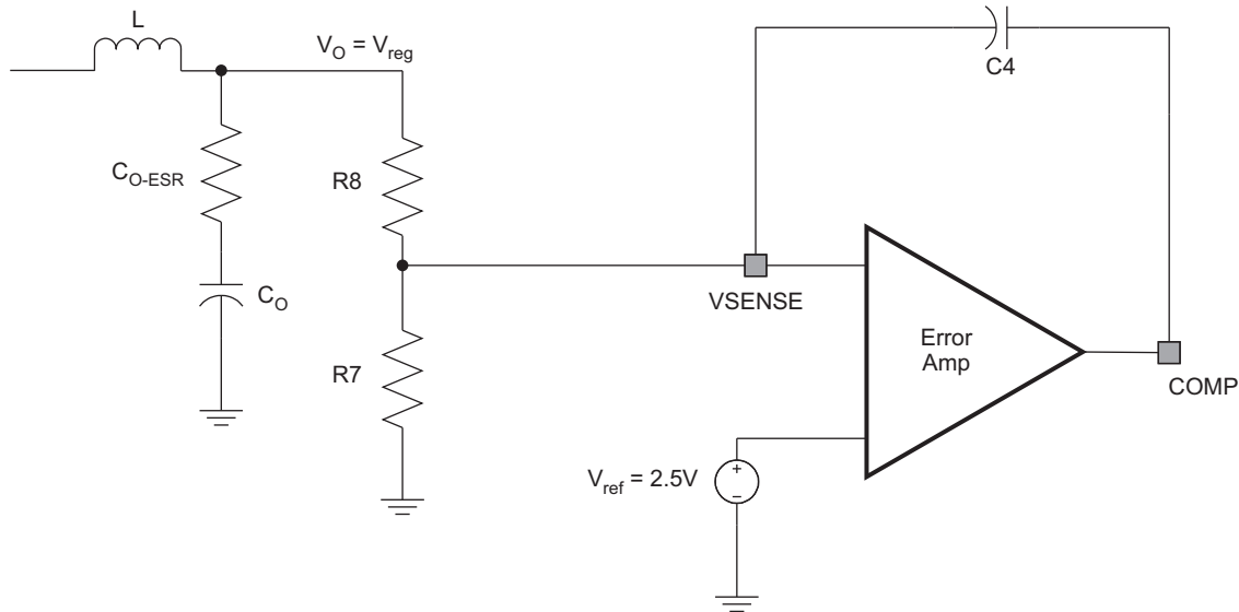
Figure 9. Type 1 Compensation
