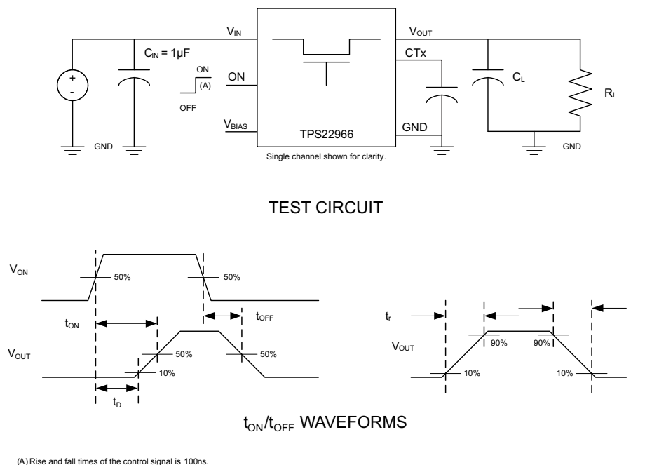
Figure 31. Test Circuit and T_{ON}/T_{OFF} Waveforms
