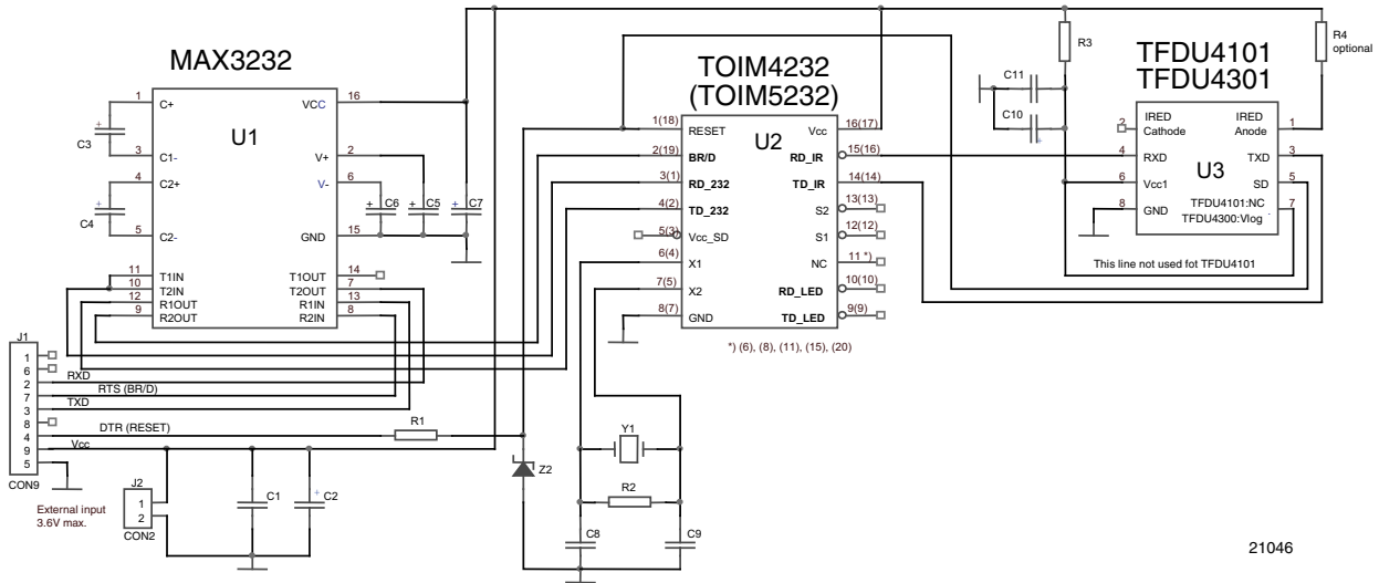
Fig. 1 - Circuit Diagram of the Demo Board
