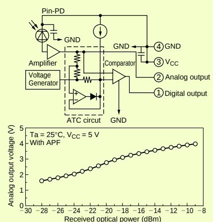
Receiving module with analog output for optical flux monitoring
