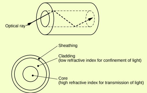
Structure of optical fiber cable
