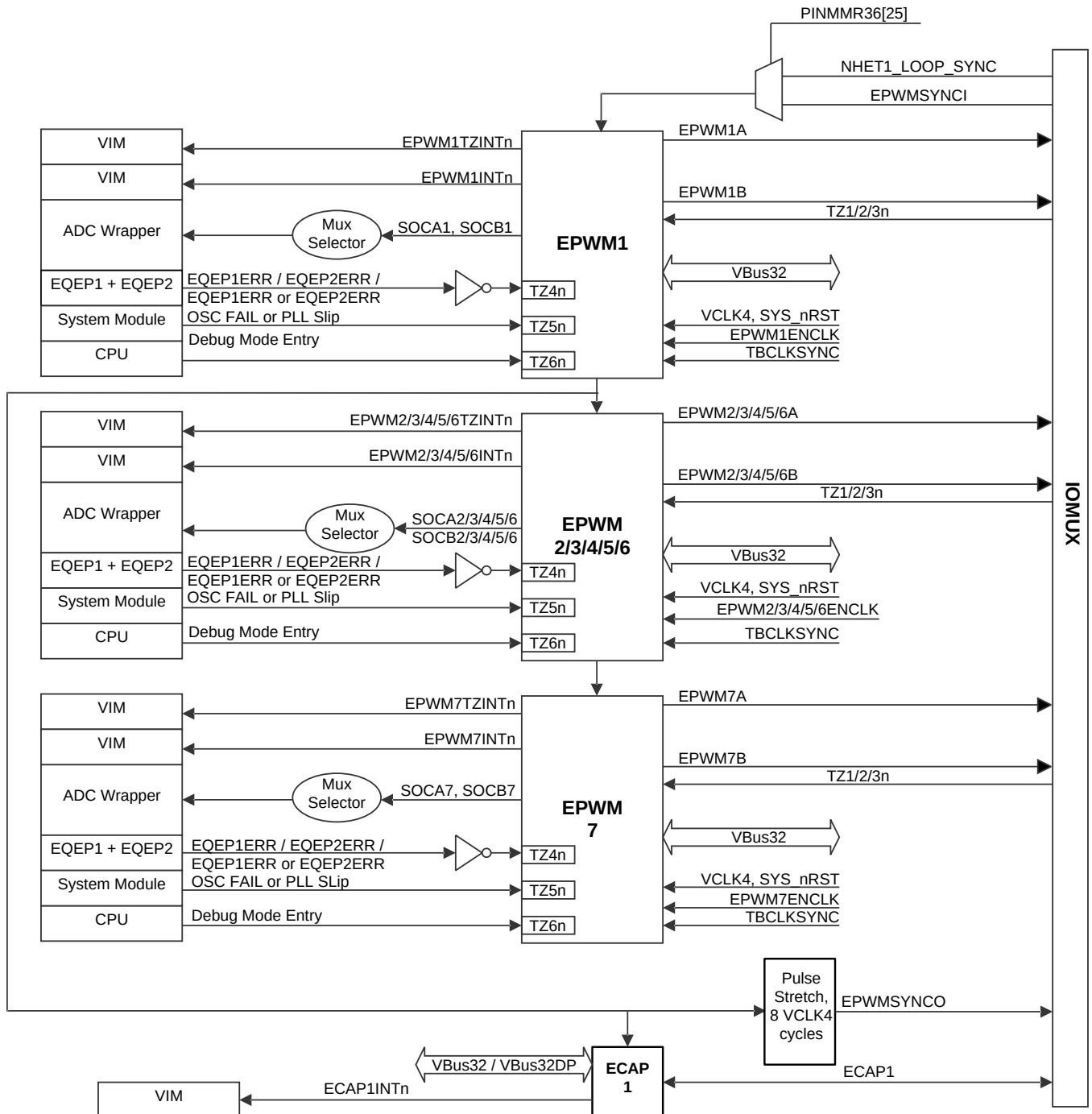
Figure 7-3. ePWMx Module Interconnections
