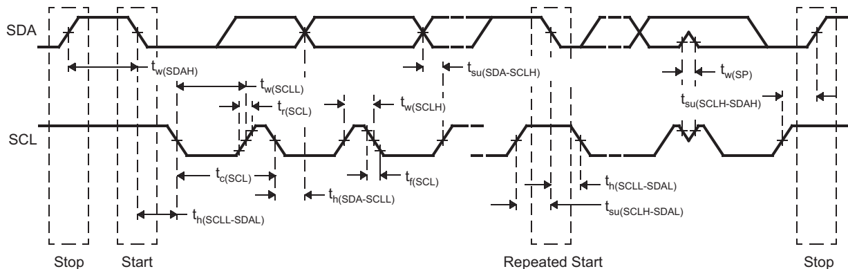
Figure 7-15. I2C Timings
