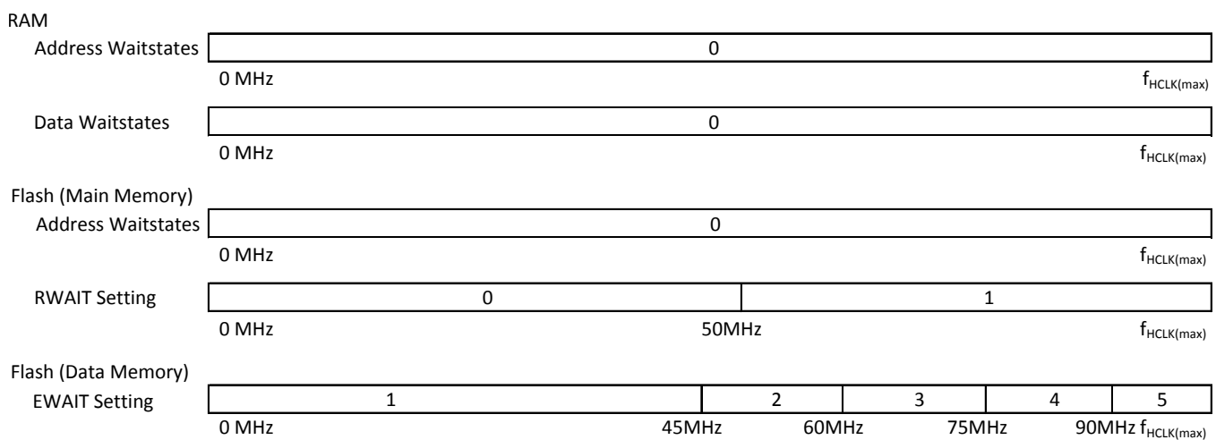
Figure 5-3. Wait States Scheme — PZ, 100 MHz
