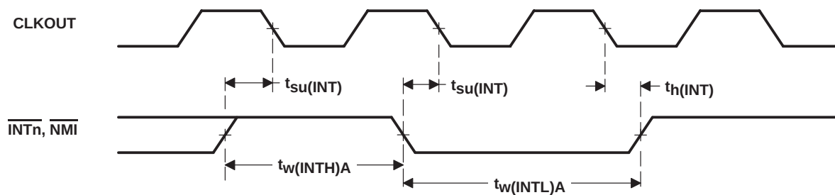
Figure 5-13. Interrupt Timing
