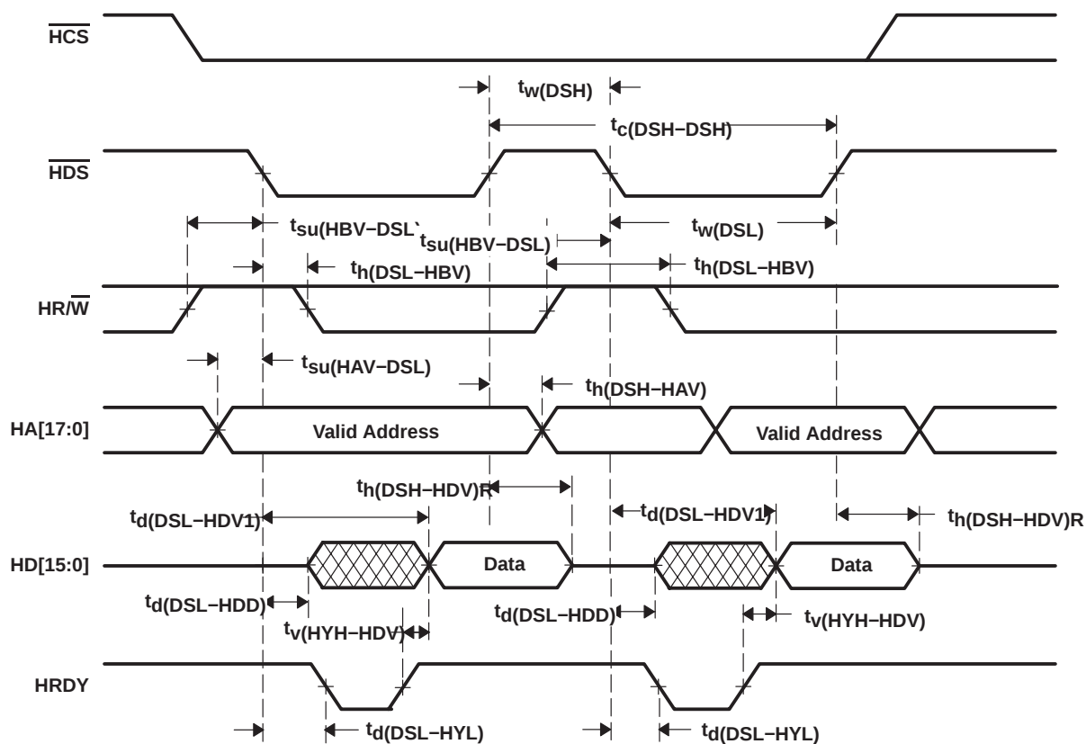
Figure 5-31. Nonmultiplexed Read Timings
