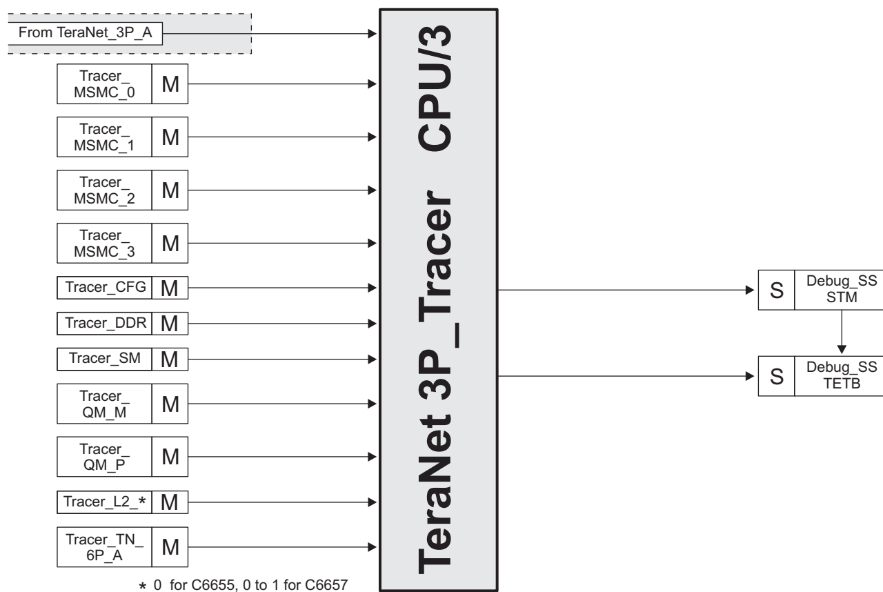
Figure 4-4 TeraNet 3P_Tracer
