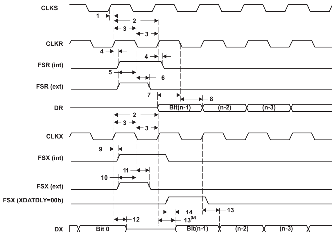
Figure 8-49. McBSP Timing
