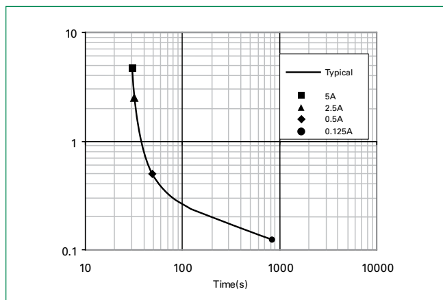
Figure 1. Thermal Characteristics
