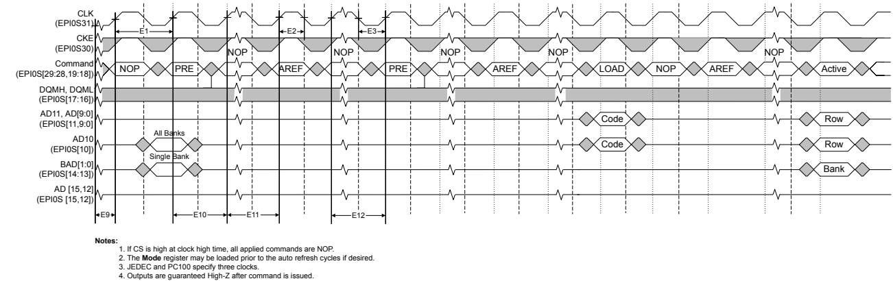
Figure 30-18. SDRAM Initialization and Load Mode Register Timing
