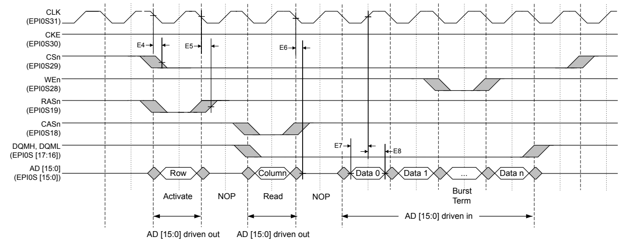
Figure 30-19. SDRAM Read Timing
