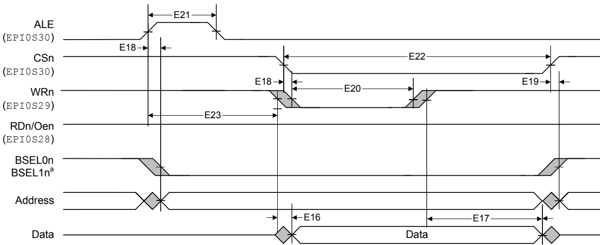
Figure 29-22. Host-Bus 8/16 Asynchronous Mode Write Timing
