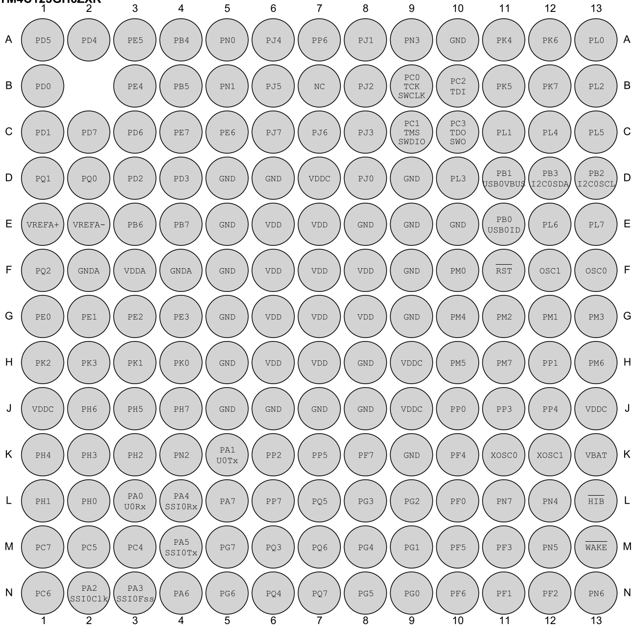
Figure 22-1. 168-Ball BGA Package Pin Diagram (Top View)
