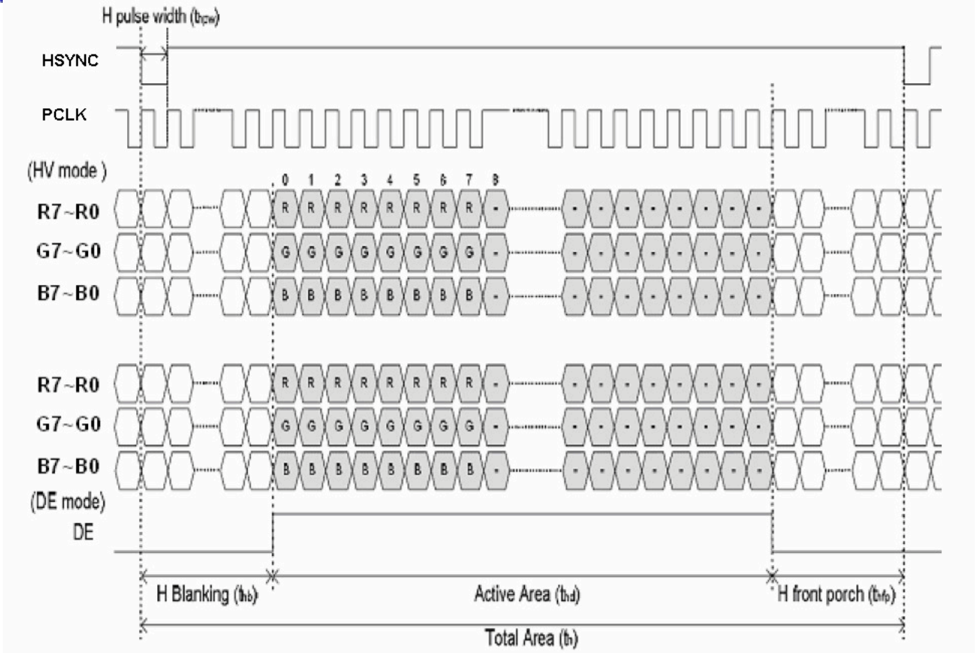
Figure 5.2 Horizontal input timing
