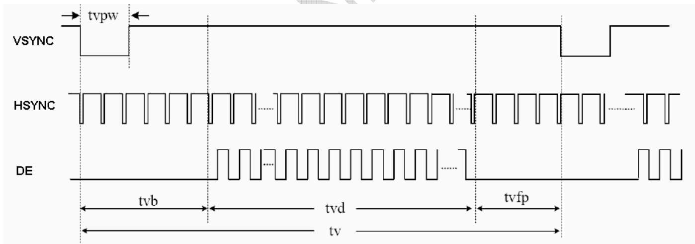
Figure 5.1 Vertical input timing
