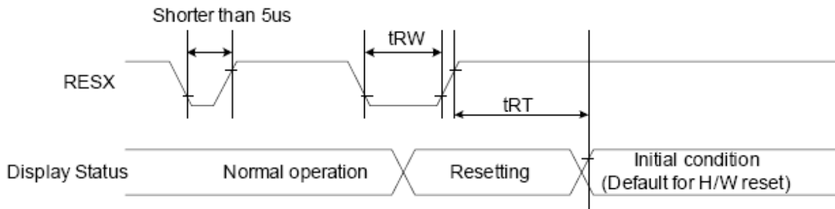
Figure 5.6.1 Reset Input Timing
