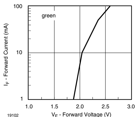
Fig. 22 - Forward Current vs. Forward Voltage
