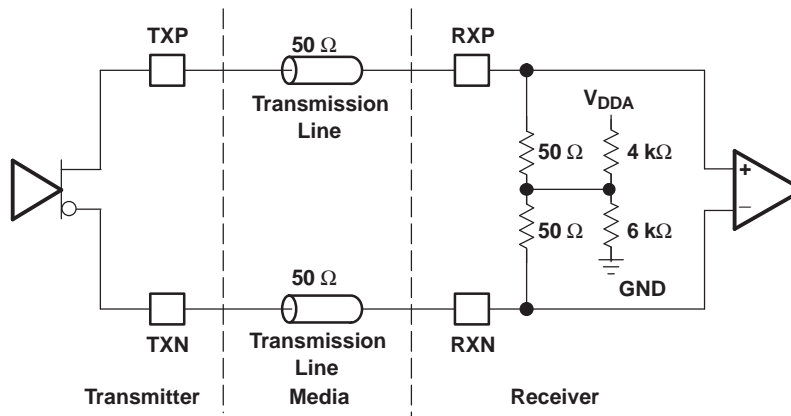
Figure 14. High-Speed I/O Directly-Coupled Mode Schematic
