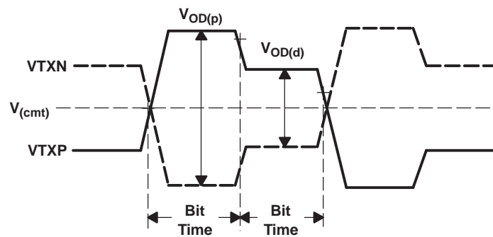
Figure 4. Common-Mode Output Voltage Definitions
