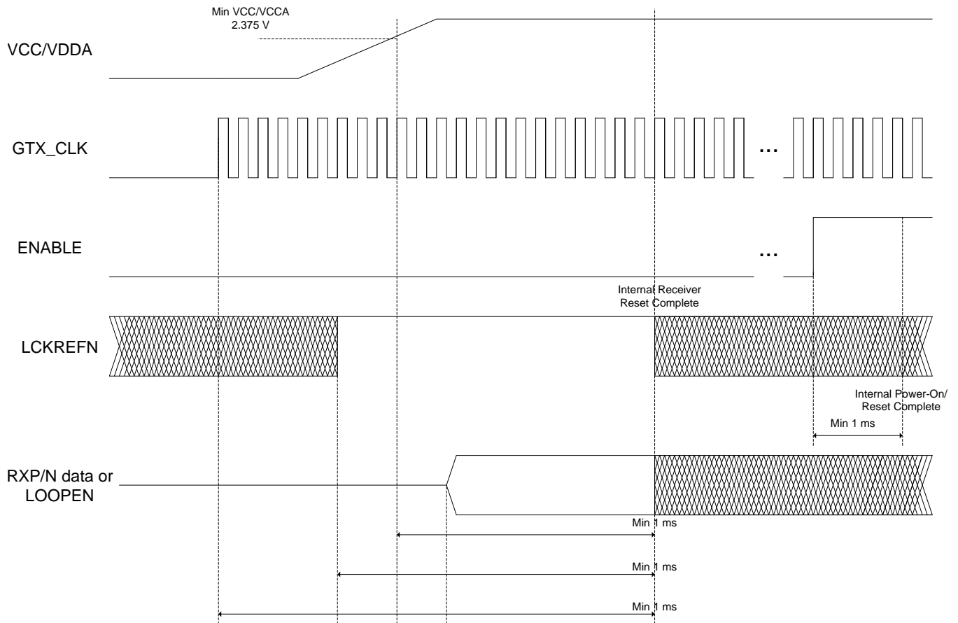
Figure 13. Power-On/Reset Timing Diagram (Option 2)
