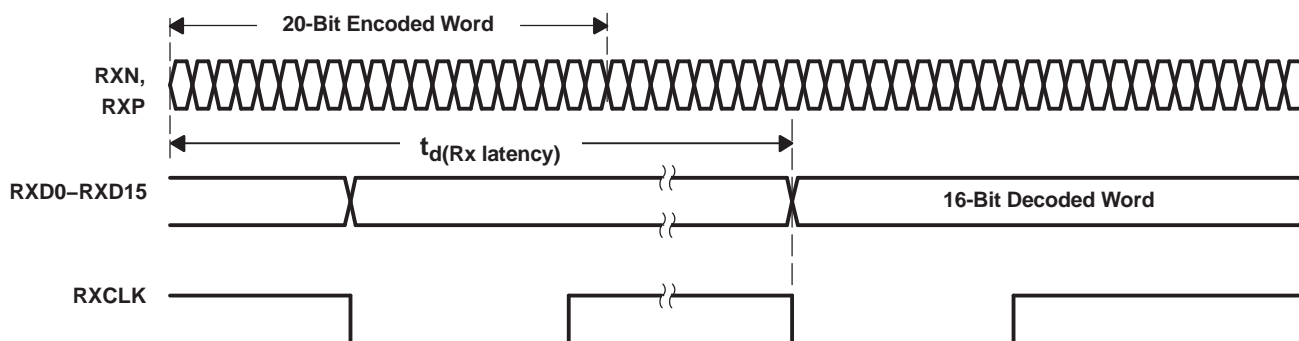
Figure 11. Receiver Latency
