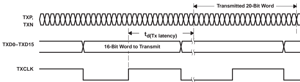
Figure 8. Transmitter Latency
