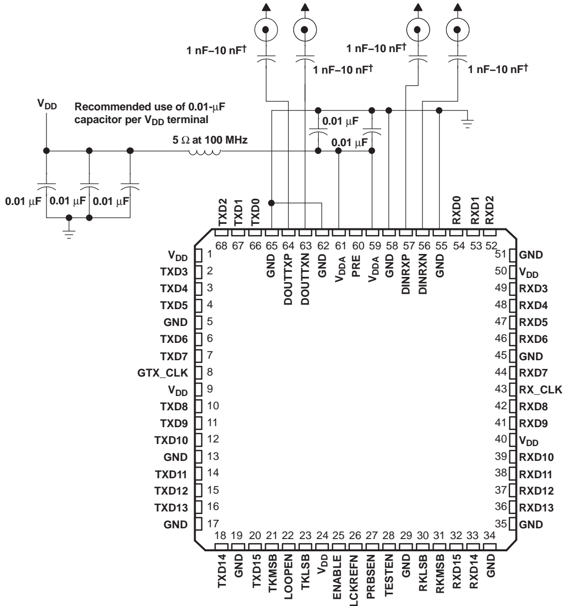
Figure 16. External Component Interconnection
