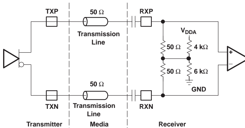
Figure 15. High-Speed I/O AC-Coupled Mode Schematic
