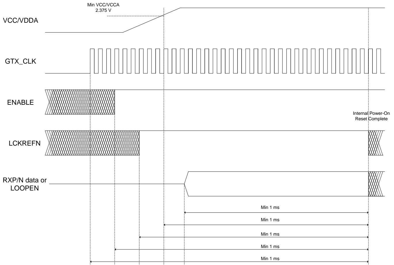
Figure 12. Power-On/Reset Timing Diagram (Option 1)
