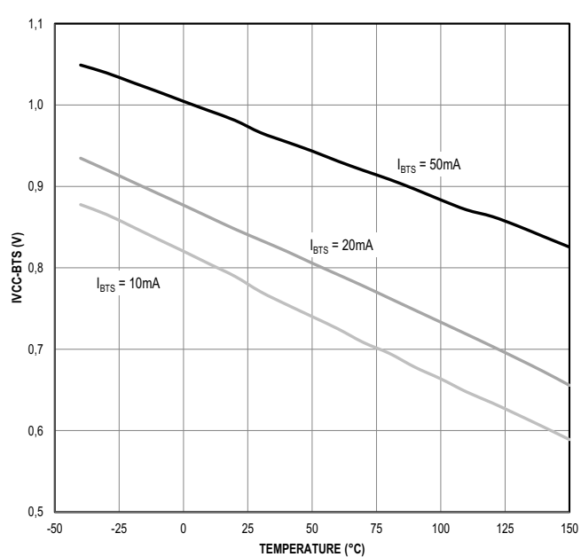
Bootstrap Diode drop versus Temperature
