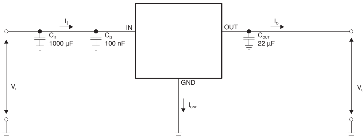
Figure 1. Test Circuit
