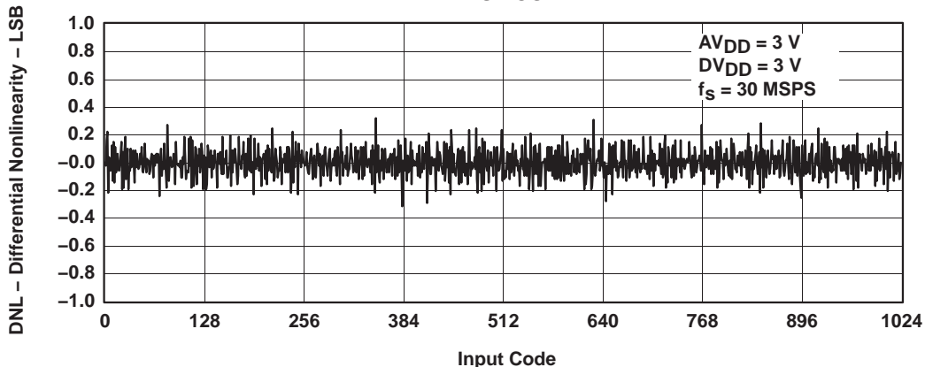
DIFFERENTIAL NONLINEARITY vs INPUT CODE
