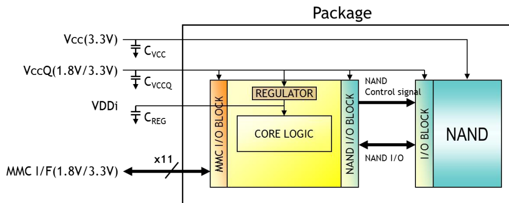
Figure 1 THGBMHG9C4LBAIR Block Diagram
