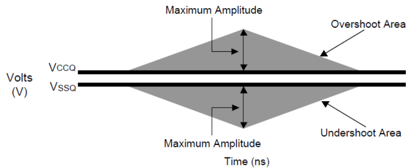
Figure 4 Overshoot/Undershoot definition
