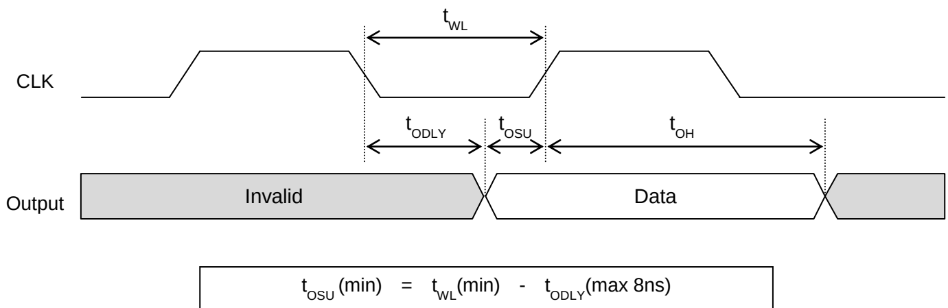
Figure 2 Output timing
