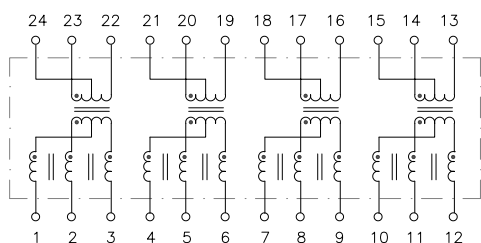
J24 Package
