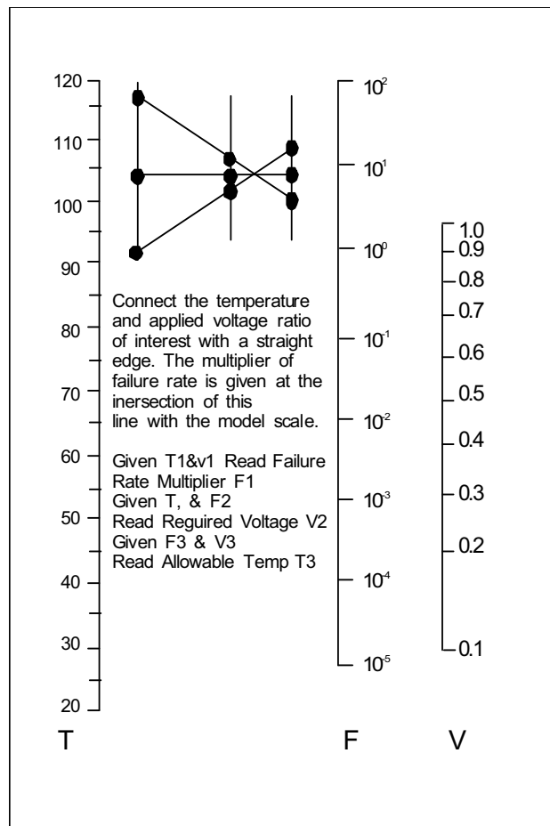
Fig.8 Reliability Nomograph
