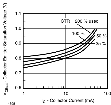
Fig. 10 - Collector Emitter Saturation Voltage vs. Collector Current
