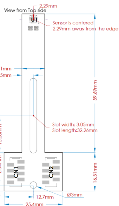
Figure 9: LT Type 1 Mechanical Drawing, mil = 0.001" = 0.0254mm
