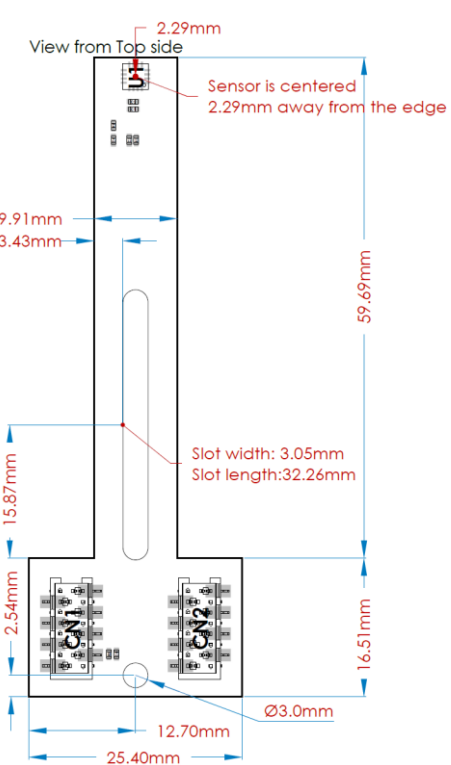
Figure 45: LT Type 5 Mechanical Drawing, mil = 0.001" = 0.0254mm
