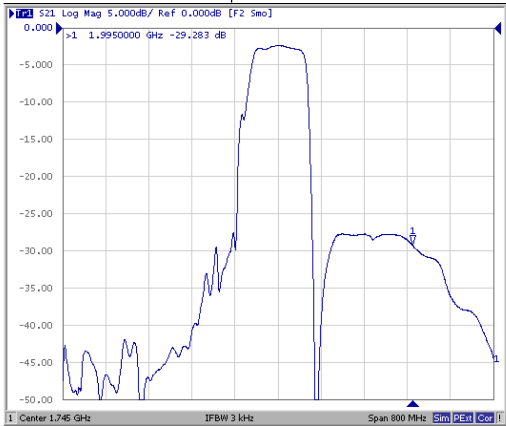
Span 800 MHz
