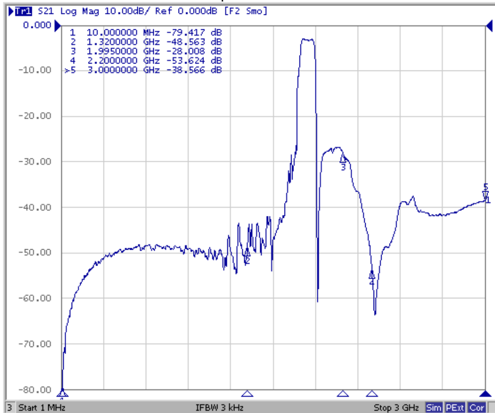
Span 3000 MHz
