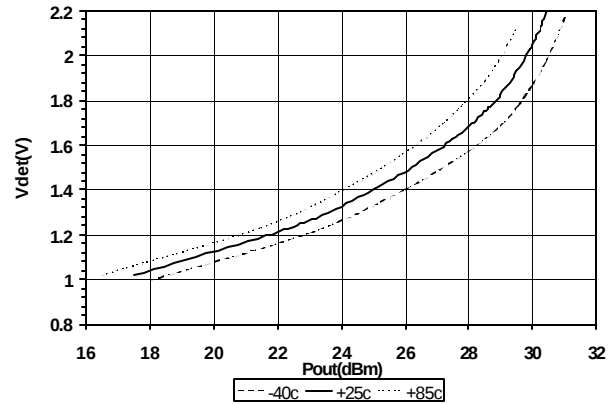
RF Power Detector (Vdet) vs Pout, F=5.35GHz
