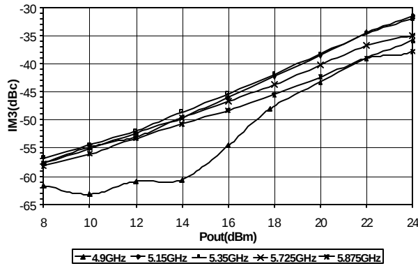
IM3 vs Pout (2 Tone Avg.), T=+25^{\circ}C Tone Spacing = 1MHz
