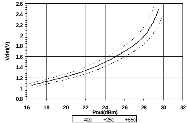
RF Power Detector (Vdet) vs Pout, F=5.875GHz
