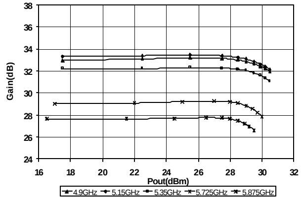
Typical Gain vs Pout, T=+25C
